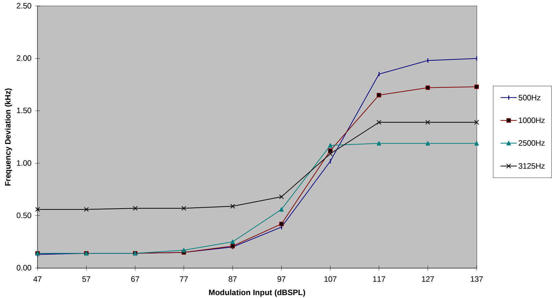
Modulation Limiting Characteristic (Model: 1010)
