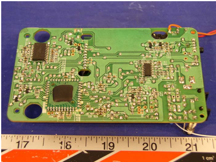
Base – Solder View
