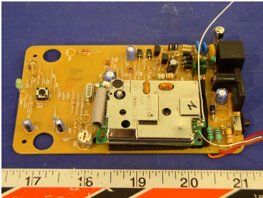
Base – Component View I
