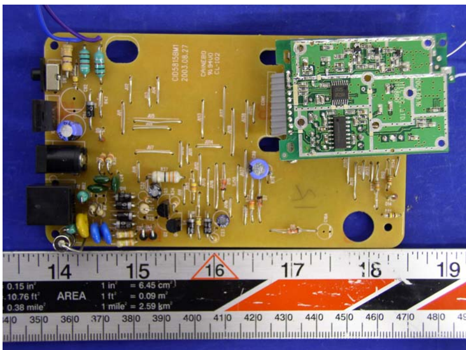
Base – Component View II
