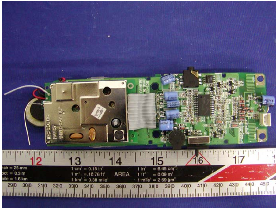
Handset – Component View I
