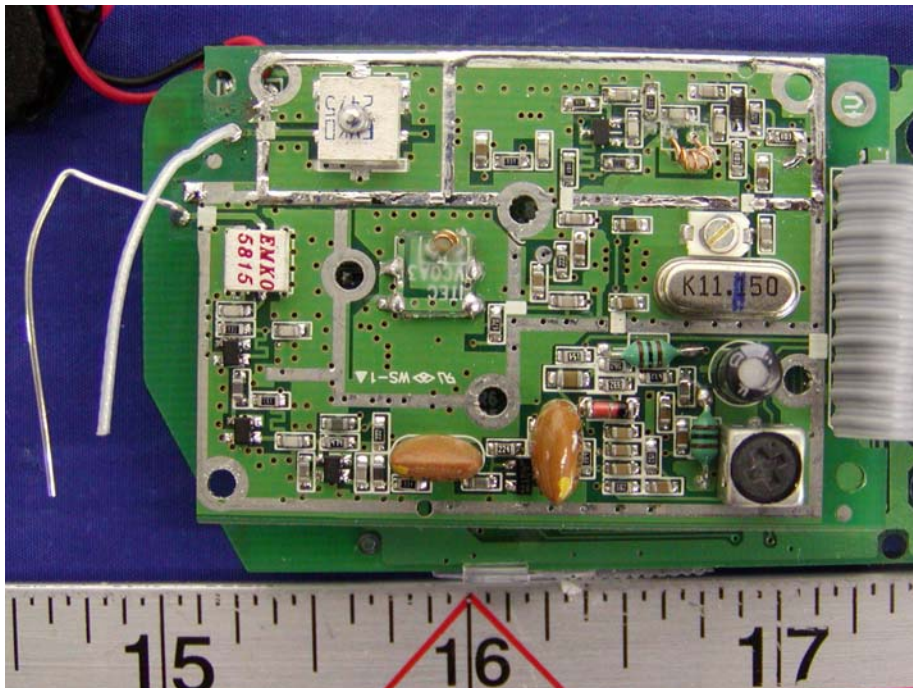
Handset Transceiver with Antenna – Top View
