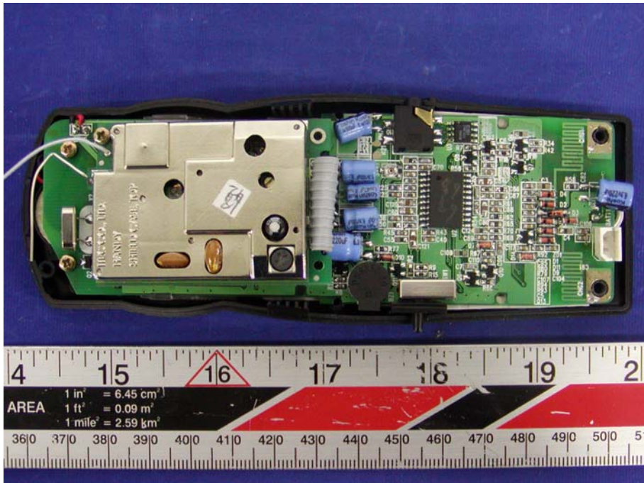
Handset – Cover Off View
