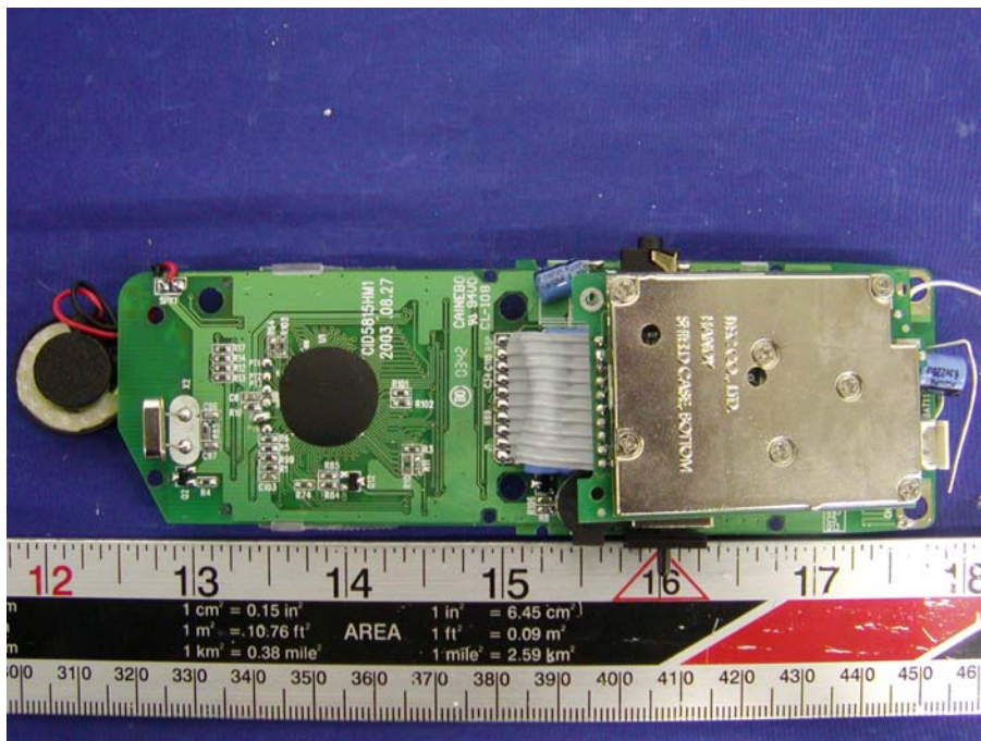
Handset – Component View II
