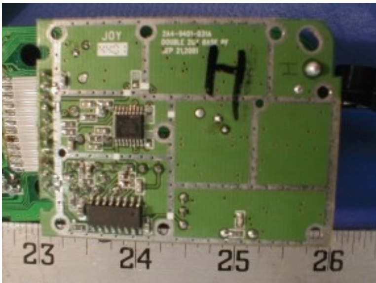
Transmitter - Solder View
