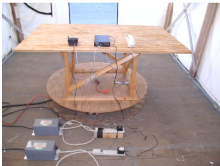
Base Conducted Emission Setup Photograph - Rear View
