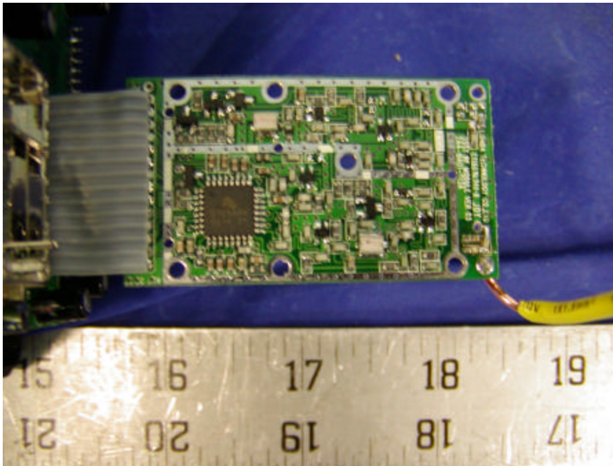
Base - Transceiver Component View
