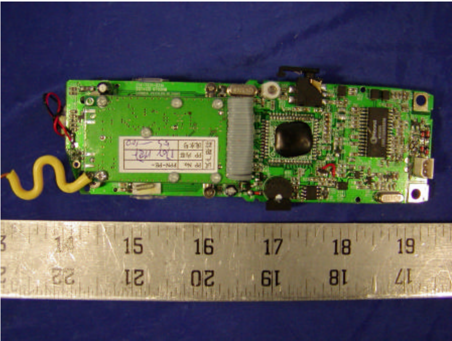
Handset - Main Board Component View
