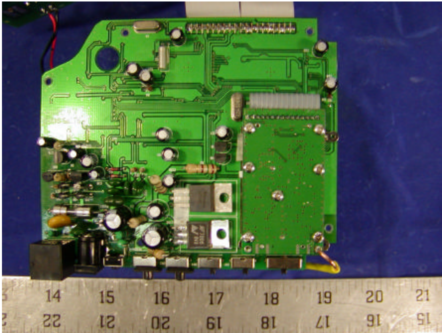
Base - Main Board Component View
