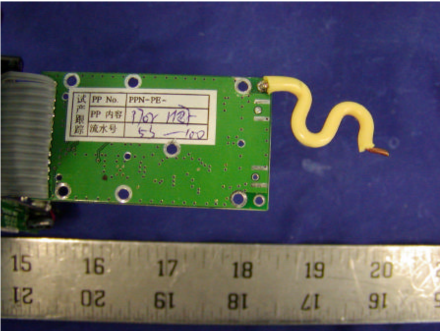
Handset - Transceiver Component View
