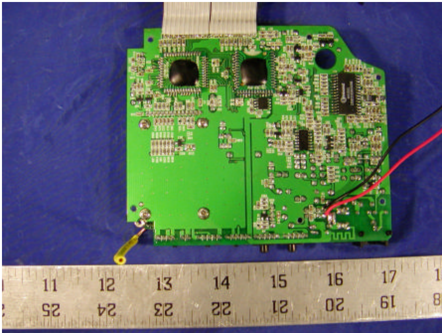
Base - Main Board Solder View
