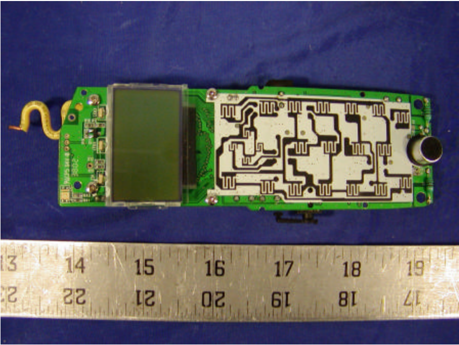
Handset - Main Board Solder View
