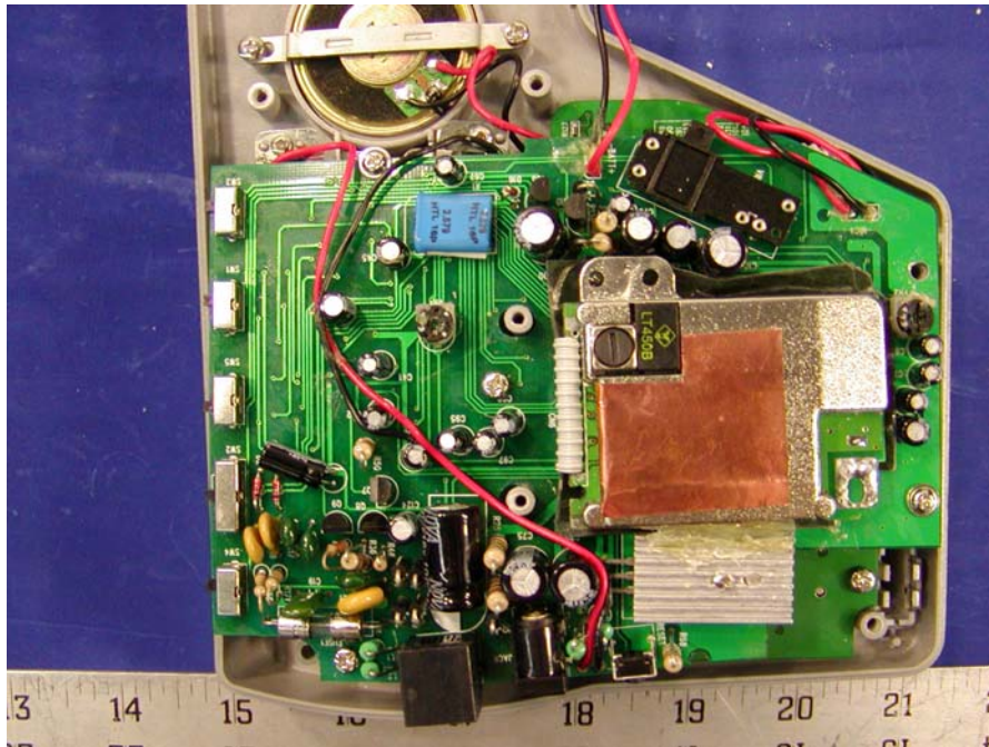
Base - Cover Off View
