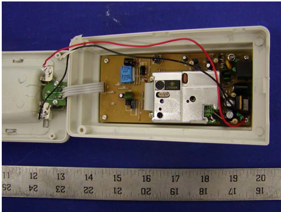
Base – Cover Off View (2)
