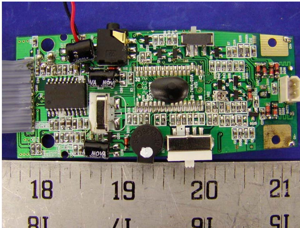
Handset - Component View
