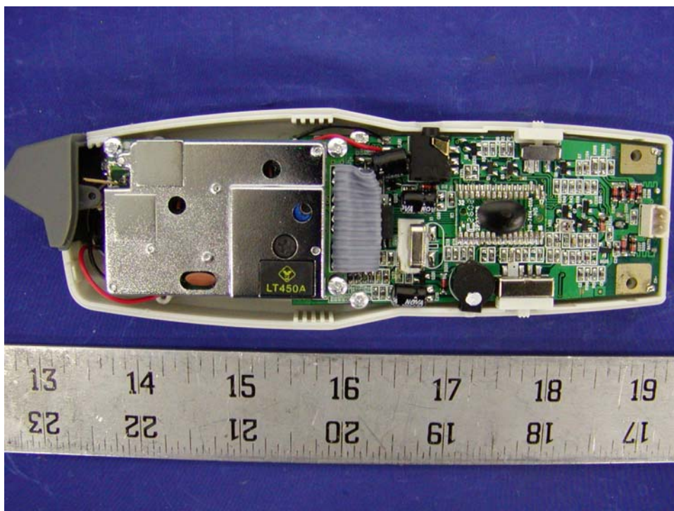
Handset – Cover Off View (2)
