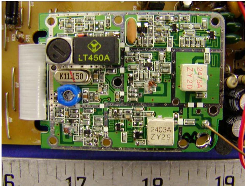
Base – Transceiver Component View
