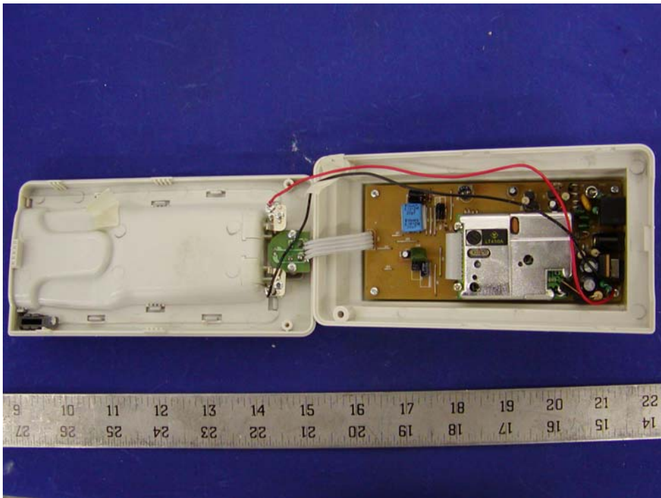
Base – Cover Off View (1)
