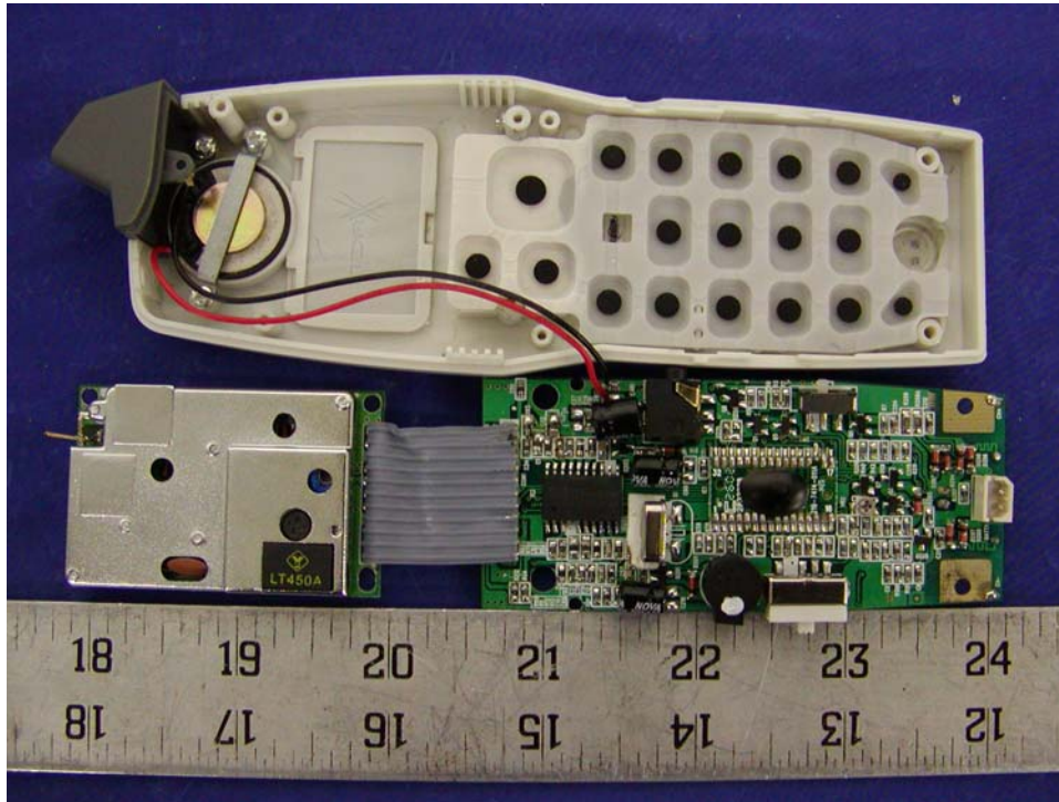
Handset – Cover Off View (1)
