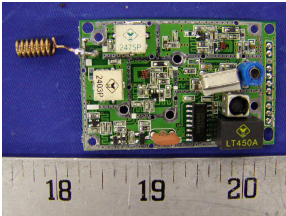
Handset – Transceiver Component View
