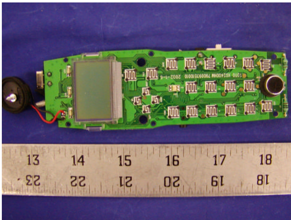
Handset – Transmitter Solder View 2
