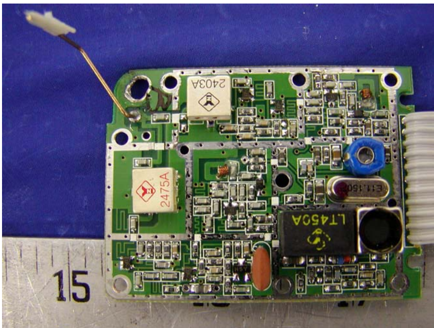
Base – Transceiver Component View
