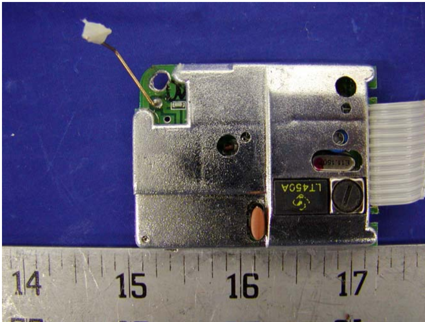
Base – Transceiver Top View
