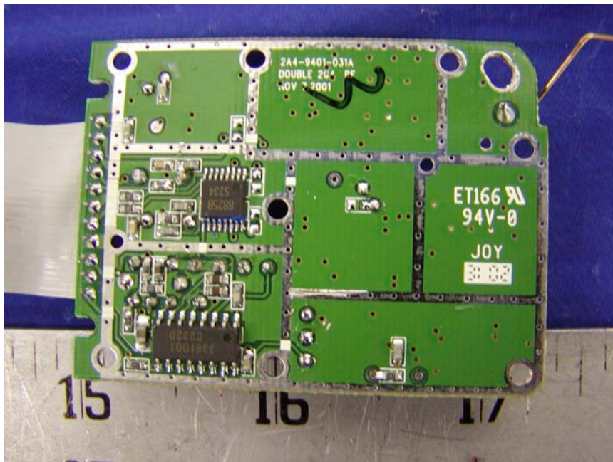
Base – Transceiver Solder View
