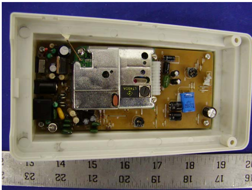
Base – Cover Off View
