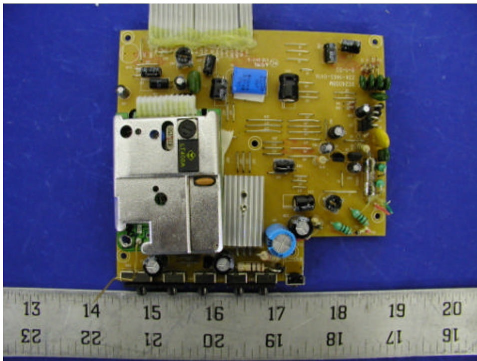
Base – Main Board Component View (1)
