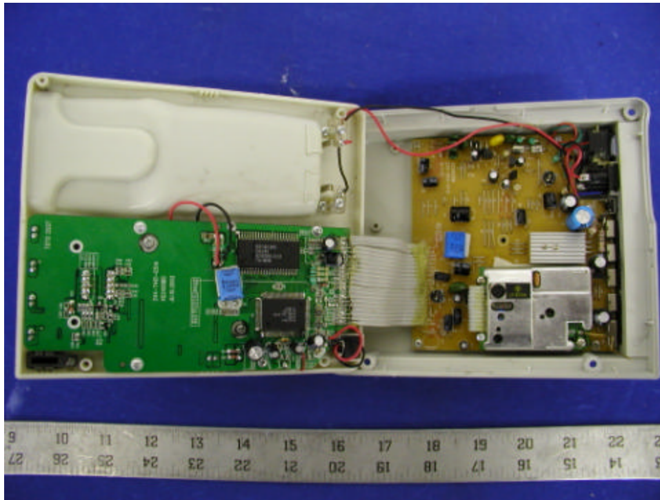
Base – Uncover View
