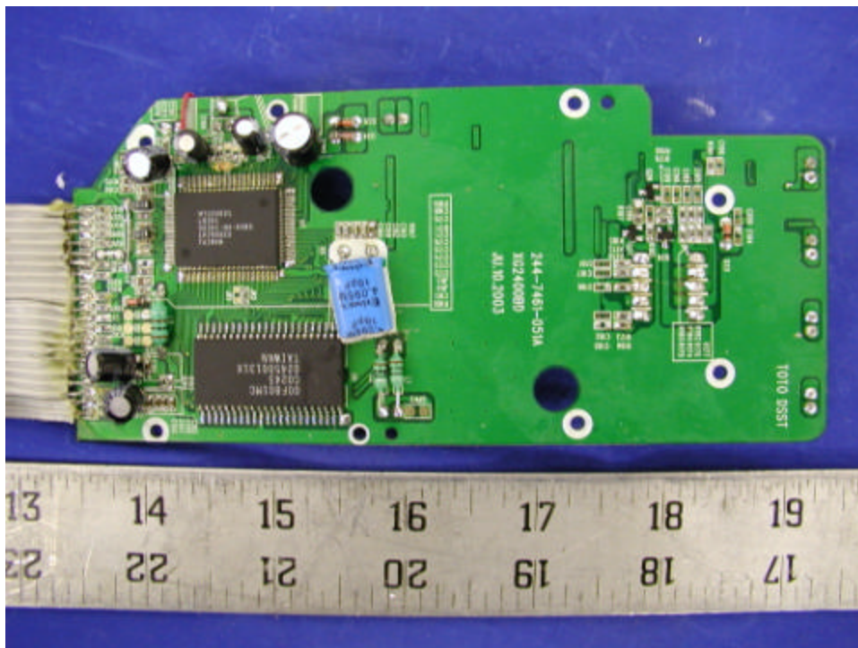
Base – Main Board Component View (2)
