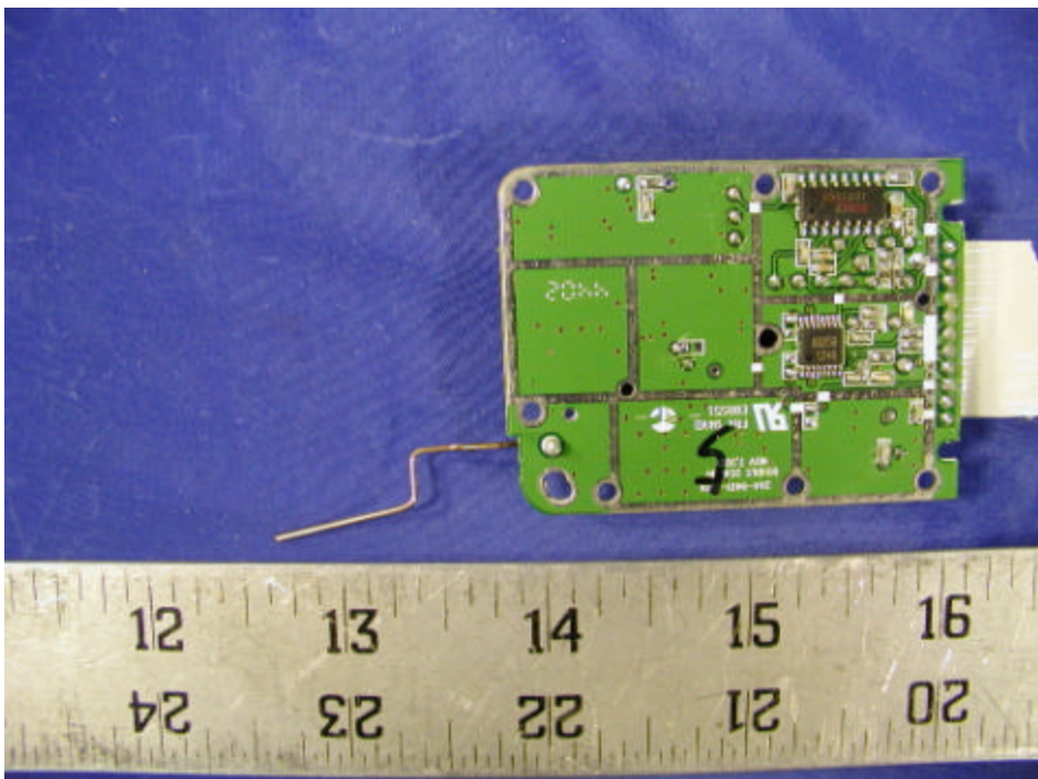
Base – Transmitter Solder View
