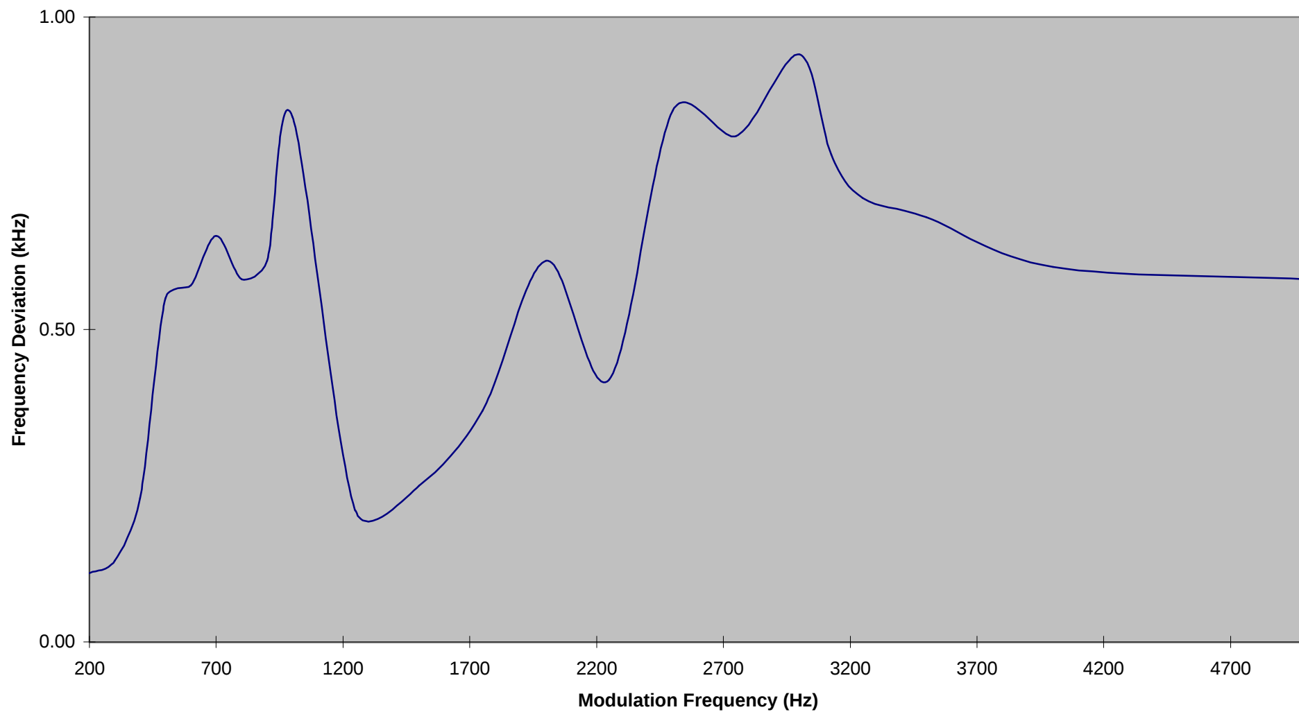
Modulation Frequency Response (Model: YURI-01)
