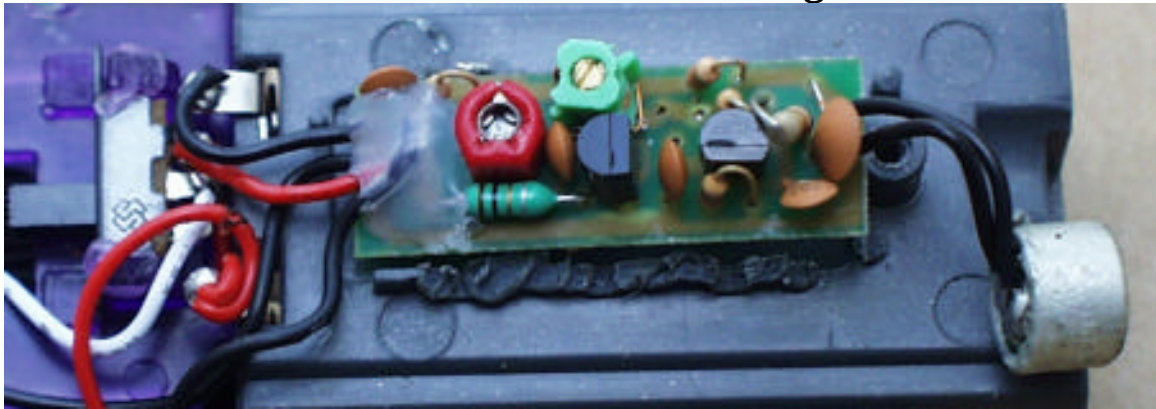
Front View of the Printed Wiring Board
