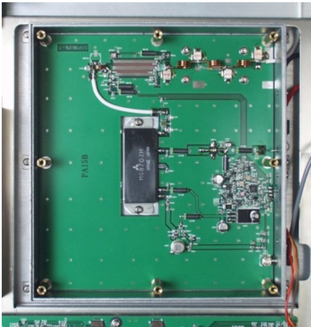
PA Interior
