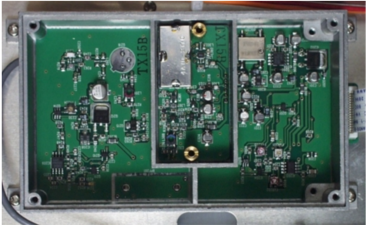
Exciter Interior
