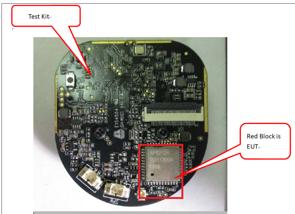
04 Rear view of PCB
