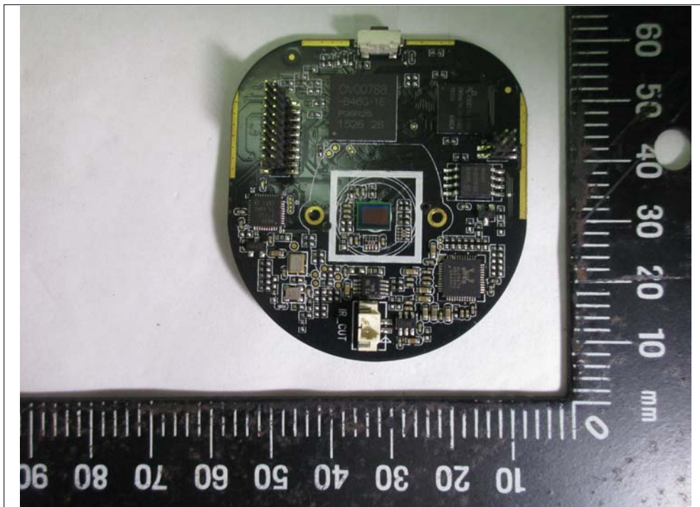
03 Front view of PCB
