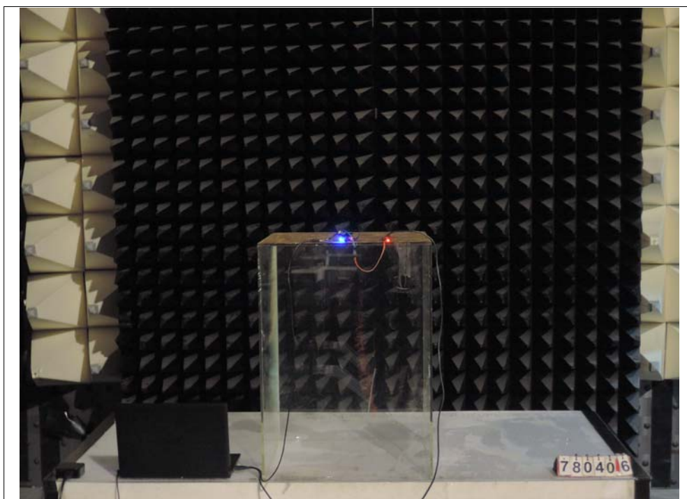
06 RE Rear View(Above 1Ghz)
