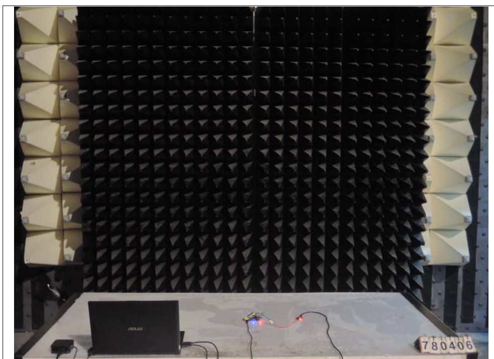
04 RE Rear View(below 1GHz)
