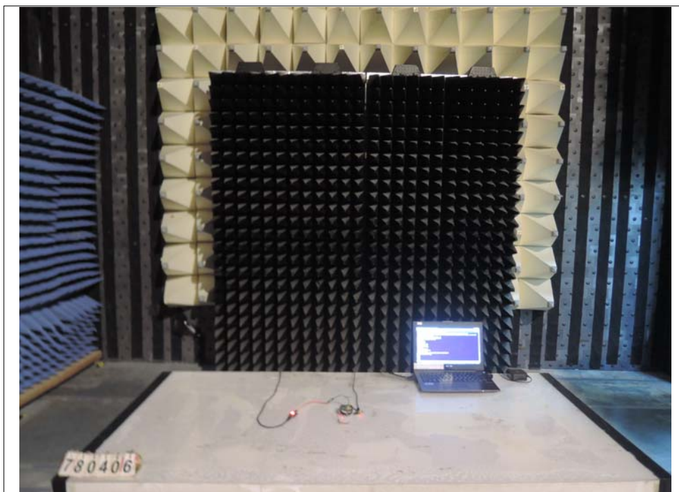
03 RE Front View (below 1GHz)
