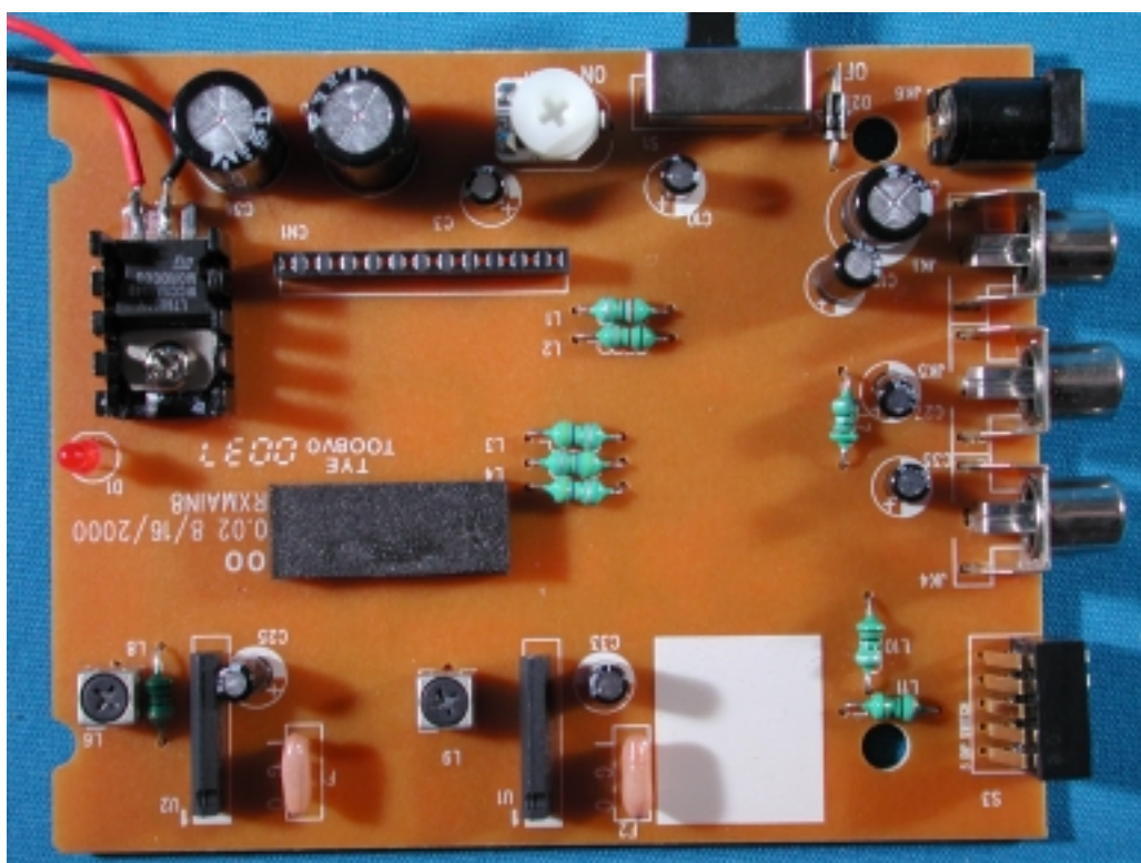
(11) EUT Photo
