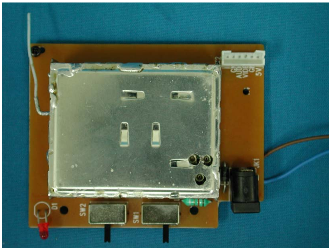
(37) EUT Photo—(Mode 2)
