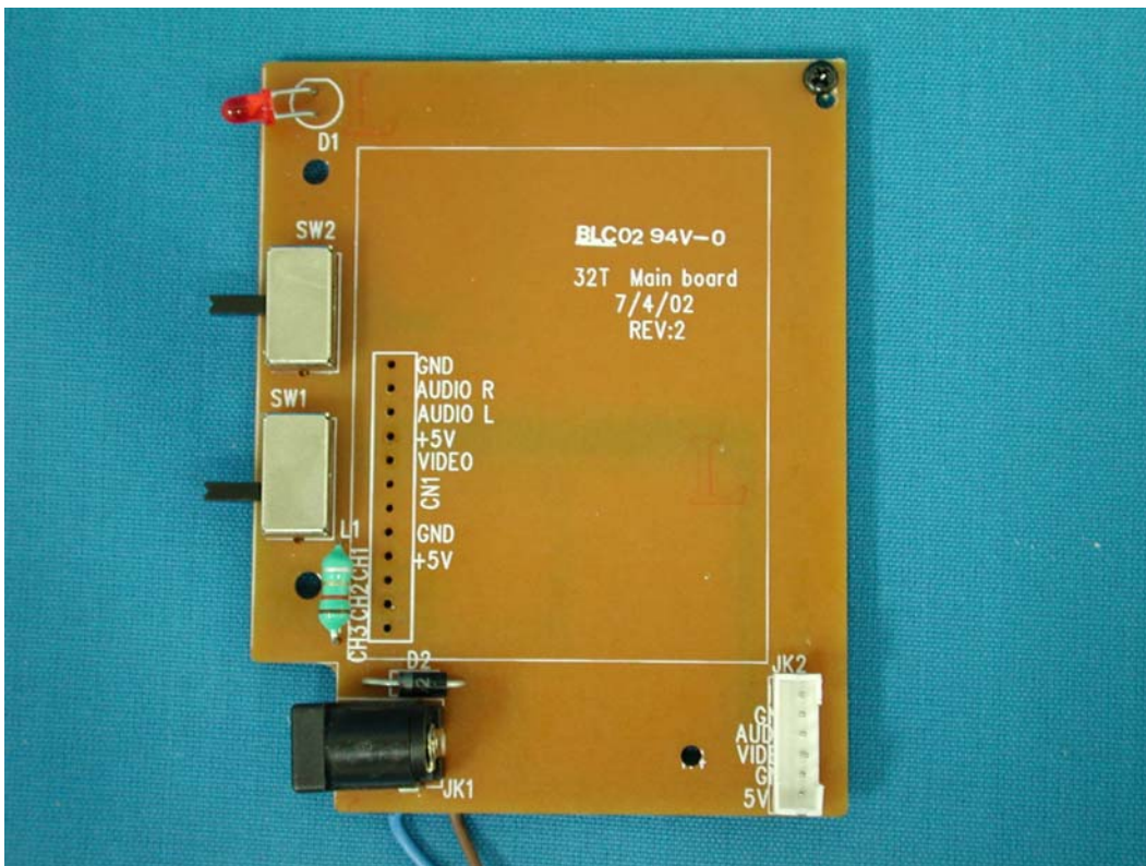
(39) EUT Photo—(Mode 2)
