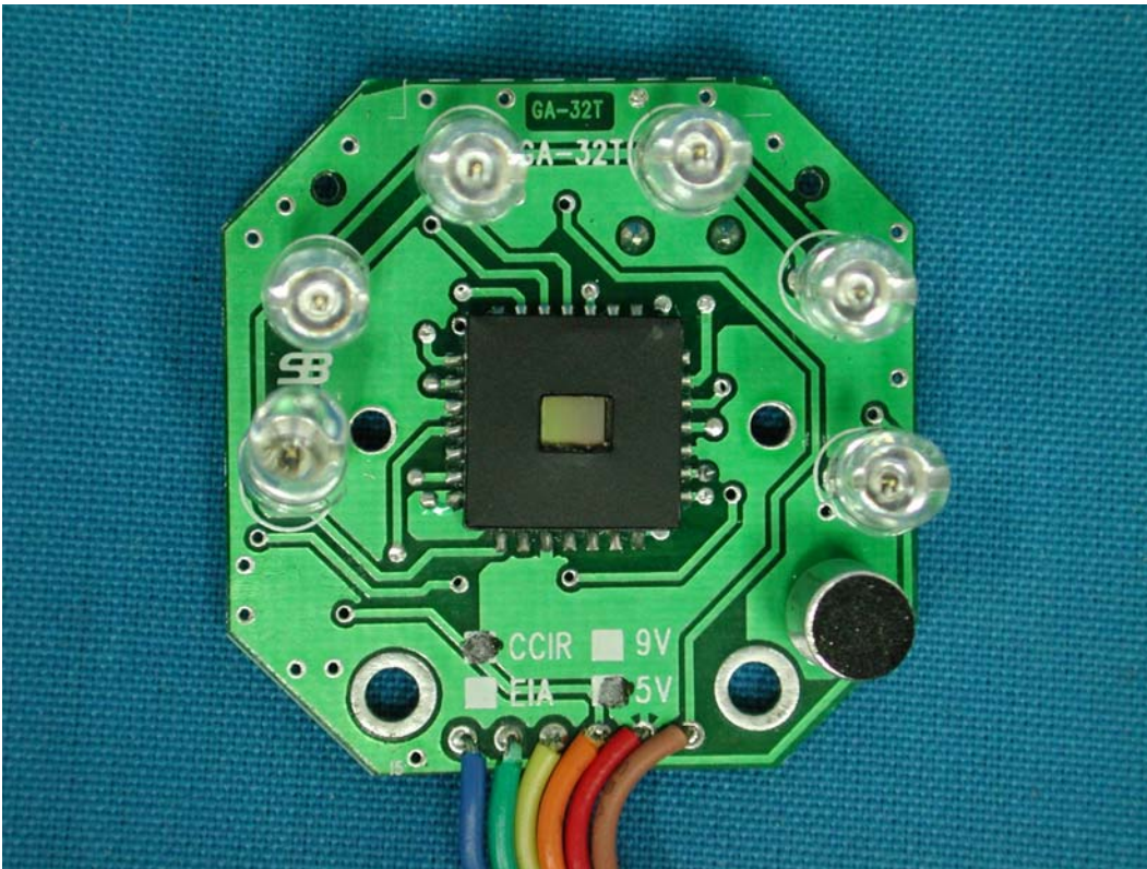
(35) EUT Photo—(Mode 2)
