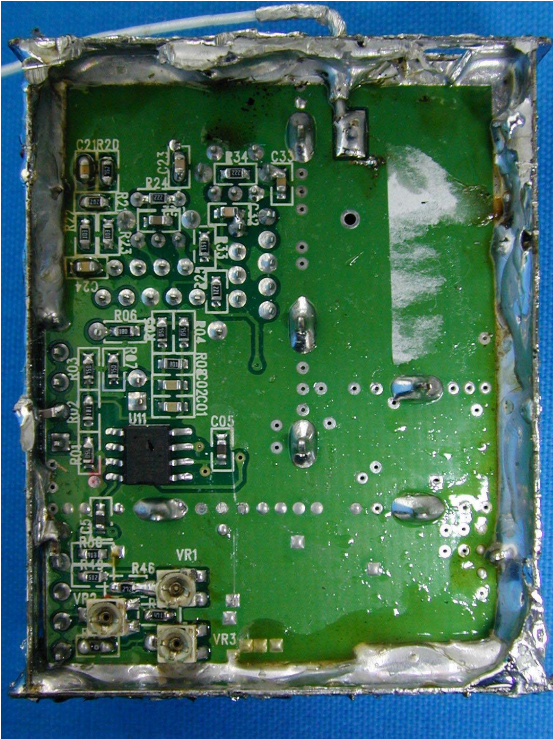
(43) EUT Photo—(Mode 2)
