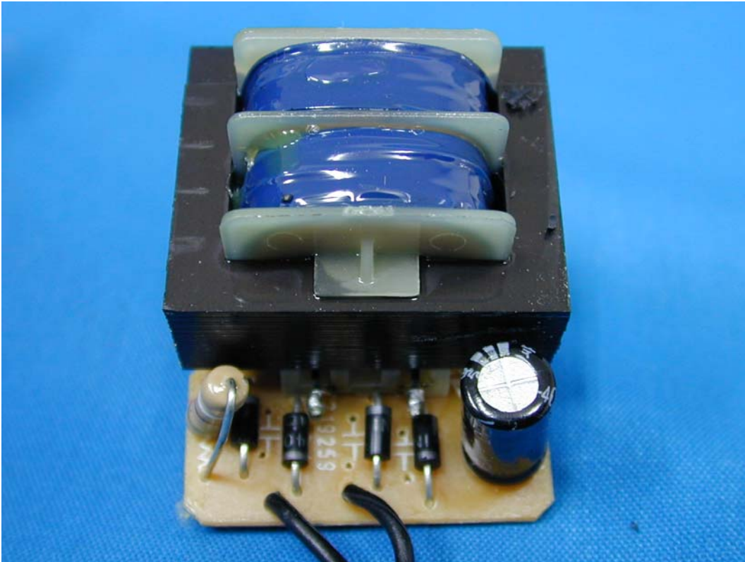
(30) EUT Photo—(Mode 2)
