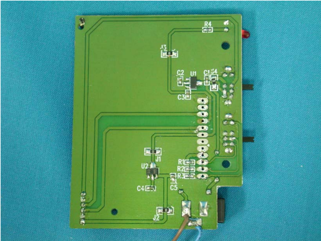
(41) EUT Photo—(Mode 2)
