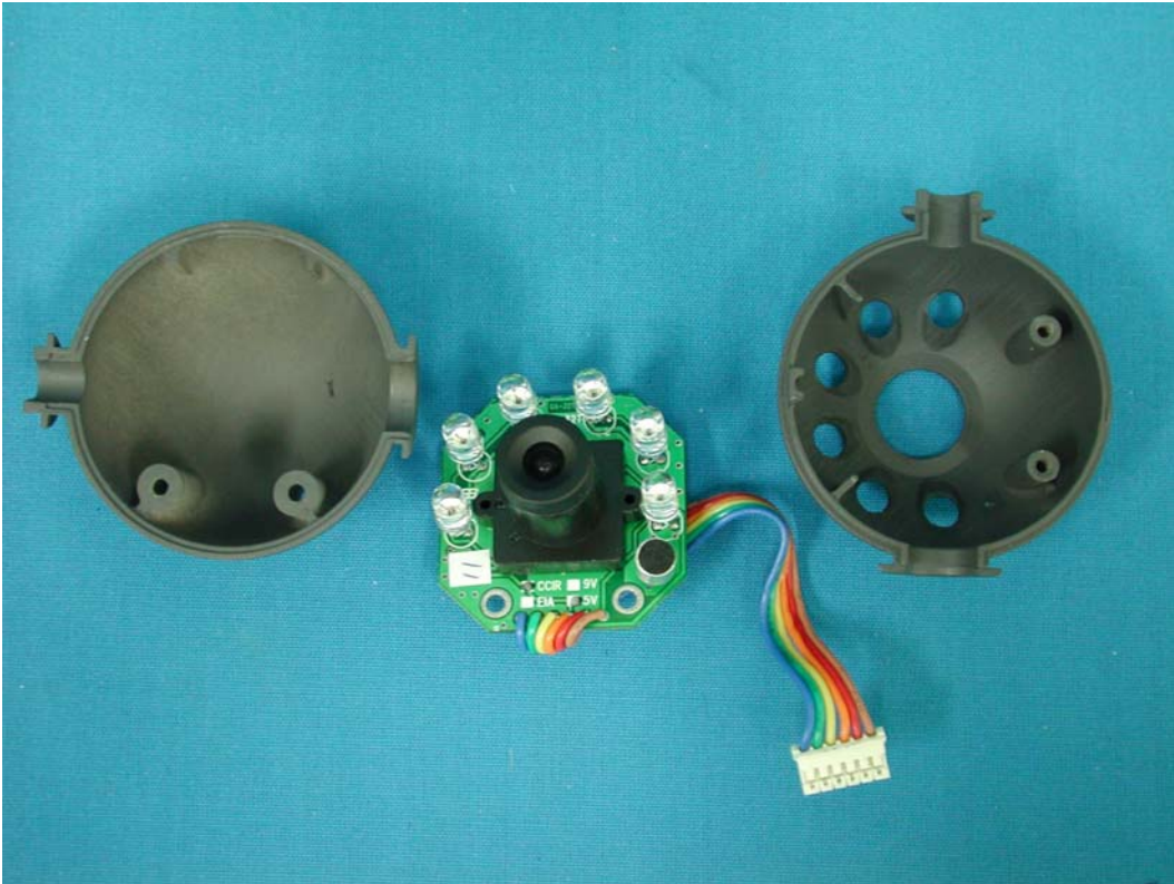
(33) EUT Photo—(Mode 2)
