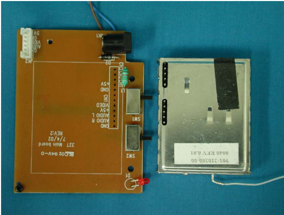
(39) EUT Photo—(Mode 2)
