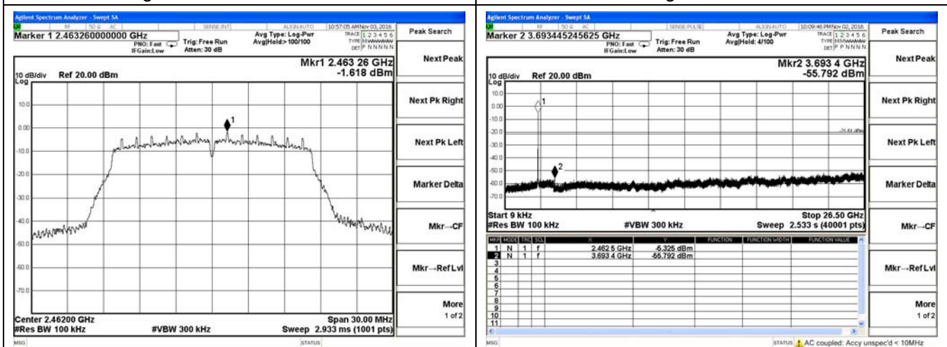
802.11g-High channel Reference
