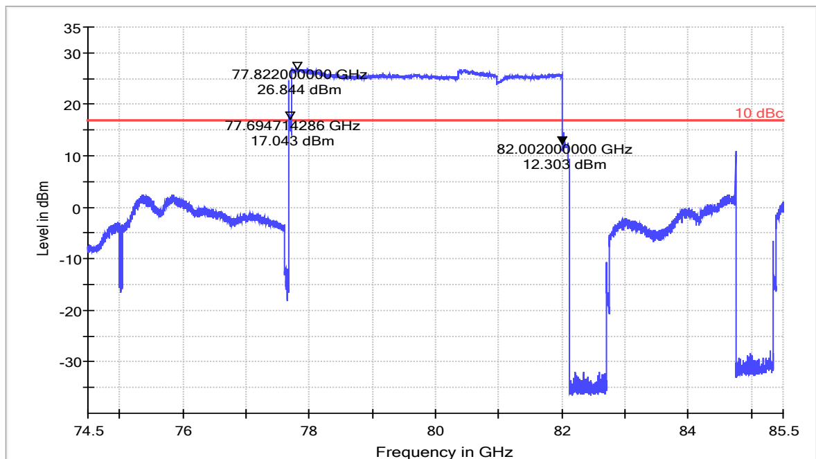
Setup_BA01
