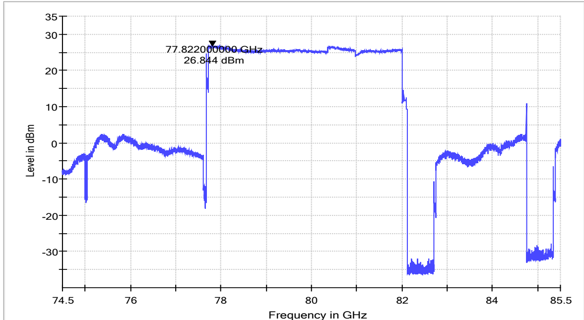
Setup_BA01 EIRP in 1 MHz
