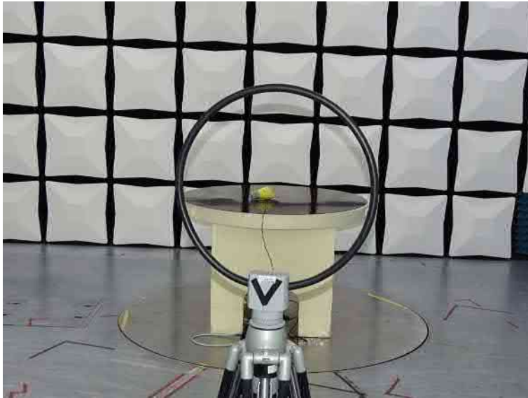
Photo 4: Test setup for radiated measurements (H-Field, CFR 47 Part 15, Subpart C, §247)
