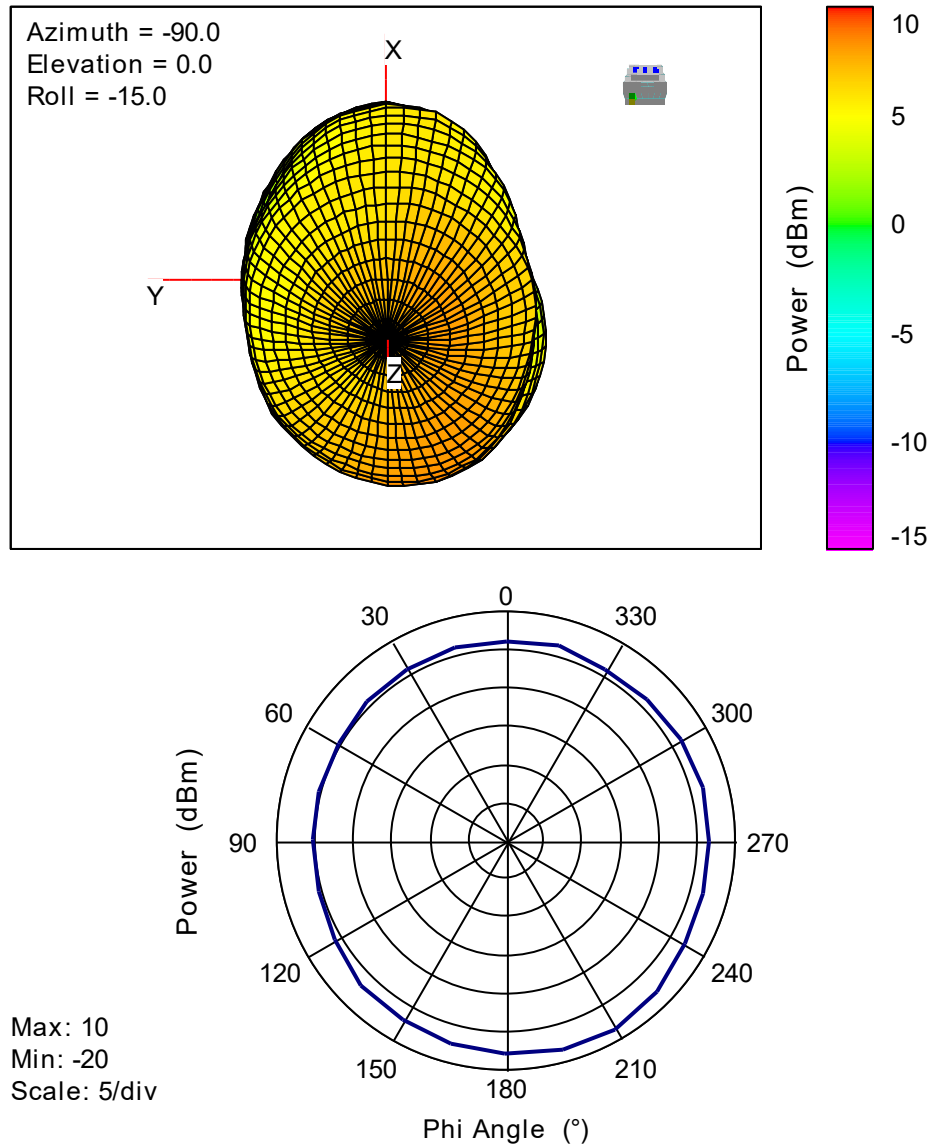
Fig. 3: 2402 MHz 3D Radiated pattern orientation of DUT.
