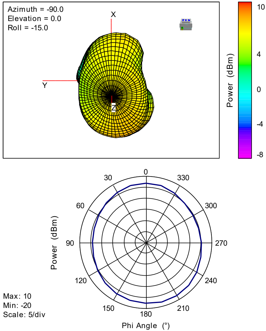
Fig. 4: 2440 MHz 3D Radiated pattern orientation of DUT.
