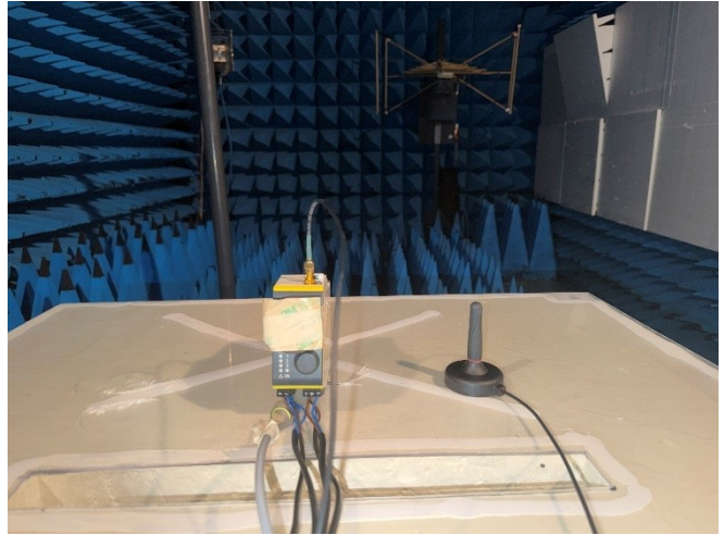
Photo in anechoic chamber – Frequency <1GHz
