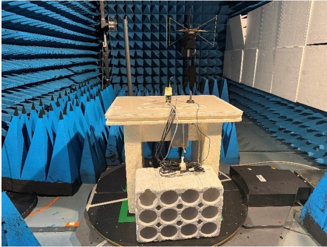
Photo in anechoic chamber – Frequency <1GHz
