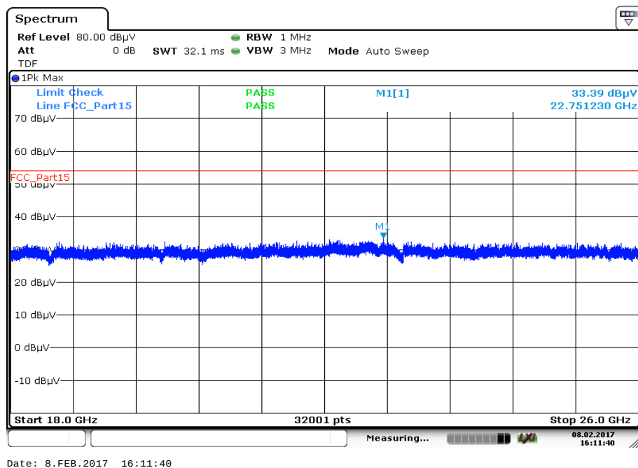
Plot 8: 18 GHz to 26 GHz, TX mode, 2440 MHz, vertical & horizontal polarization
