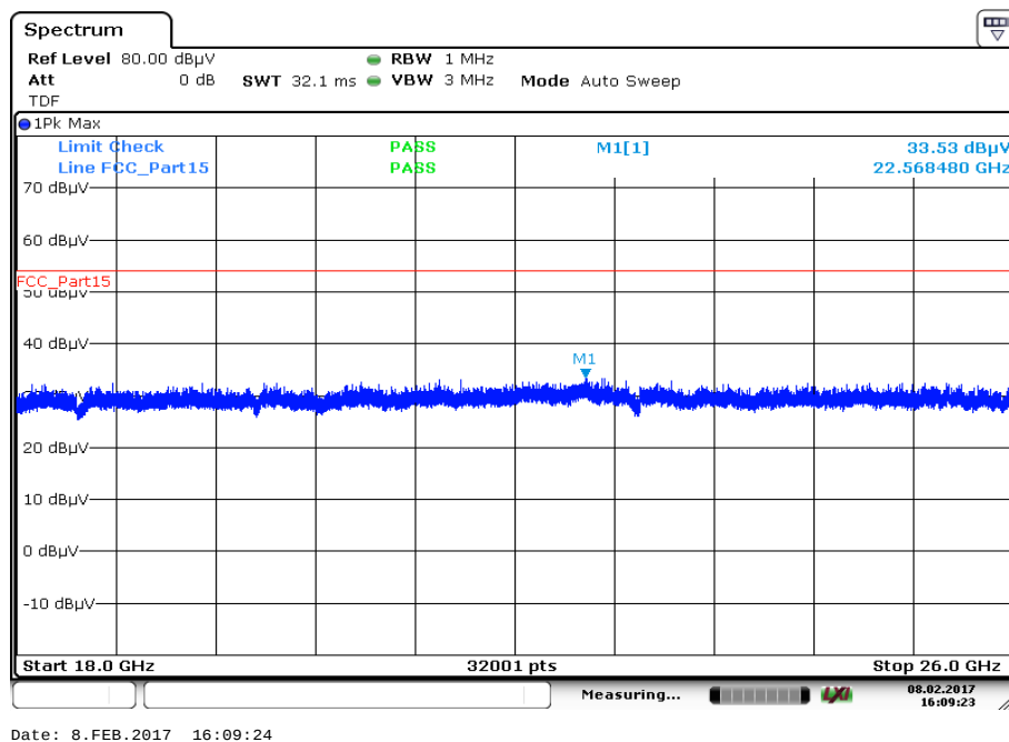
Plot 4: 18 GHz to 26 GHz, TX mode, 2402 MHz, vertical & horizontal polarization
