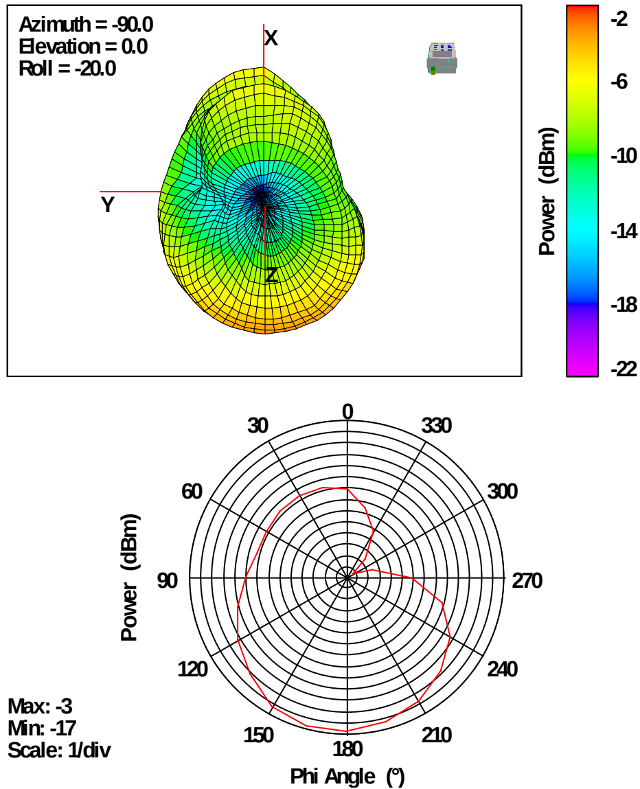
Fig. 3: 2402 MHz 3D Radiated pattern orientation of DUT compared to a phone.
