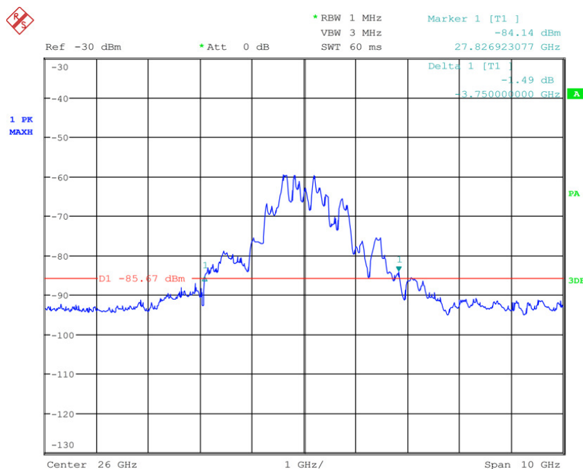
Plot 5-1: Modulated Bandwidth - TC #1
