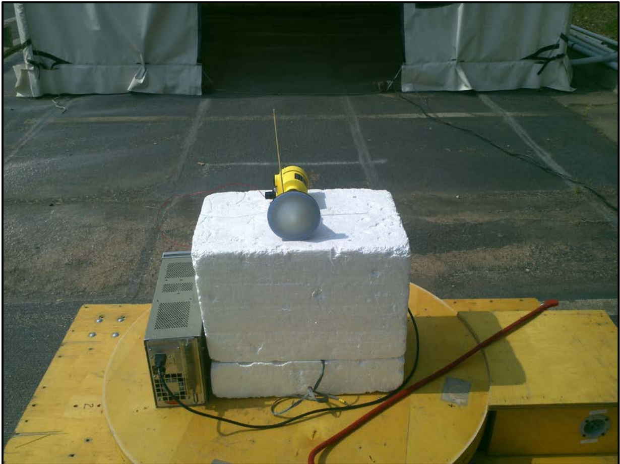
Photograph 6: Radiated Emissions – Front View - TC #1
