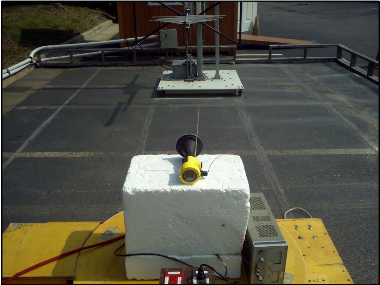
Photograph 7: Radiated Emissions – Rear View - TC #1
