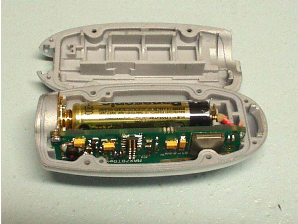
EUT Inside View with Battery
