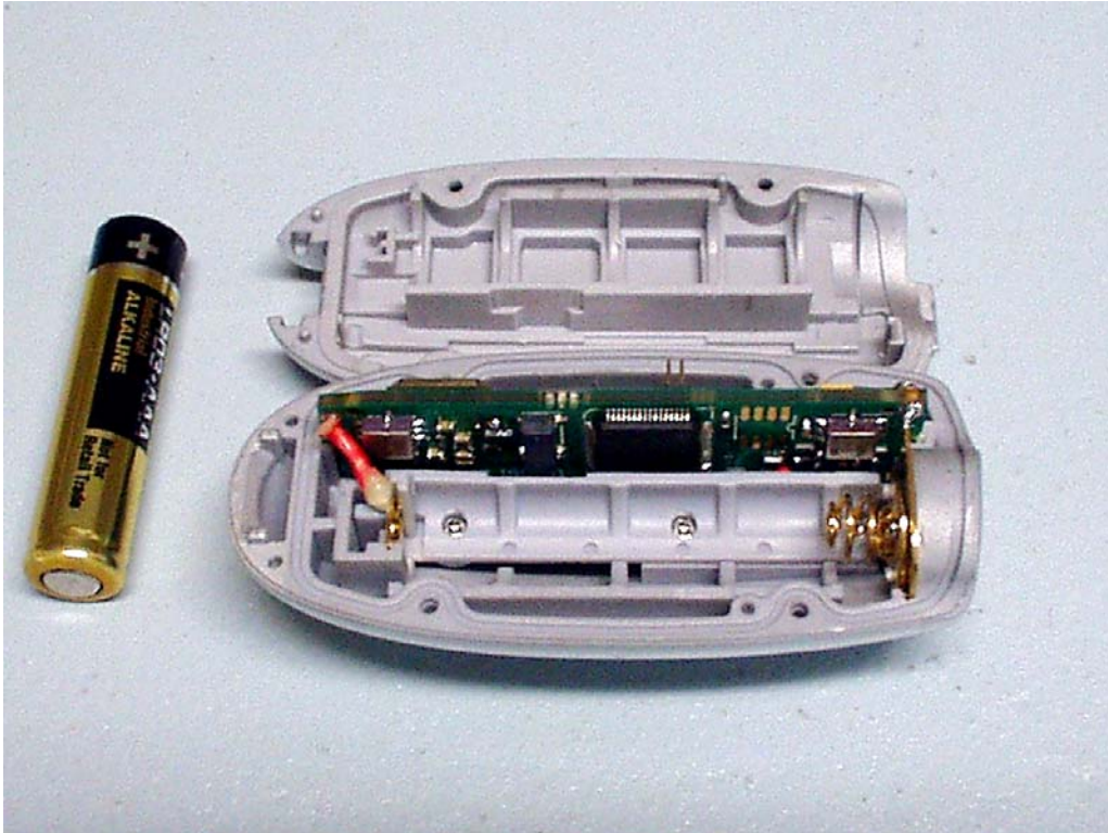
EUT Inside View without Battery
