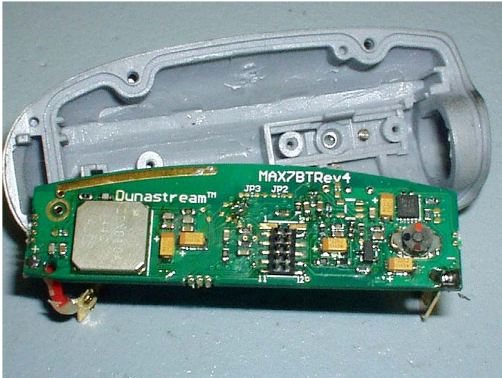
EUT Component Top View
