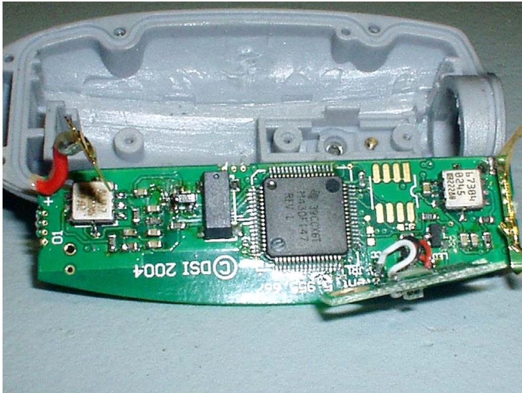
EUT Component Bottom View
