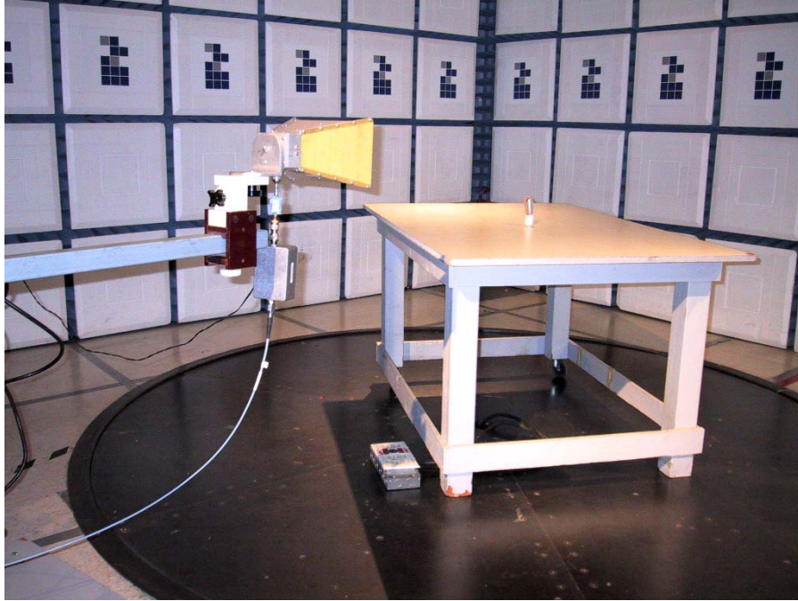
Radiated Emissions in Restricted Bands Test Set-Up
