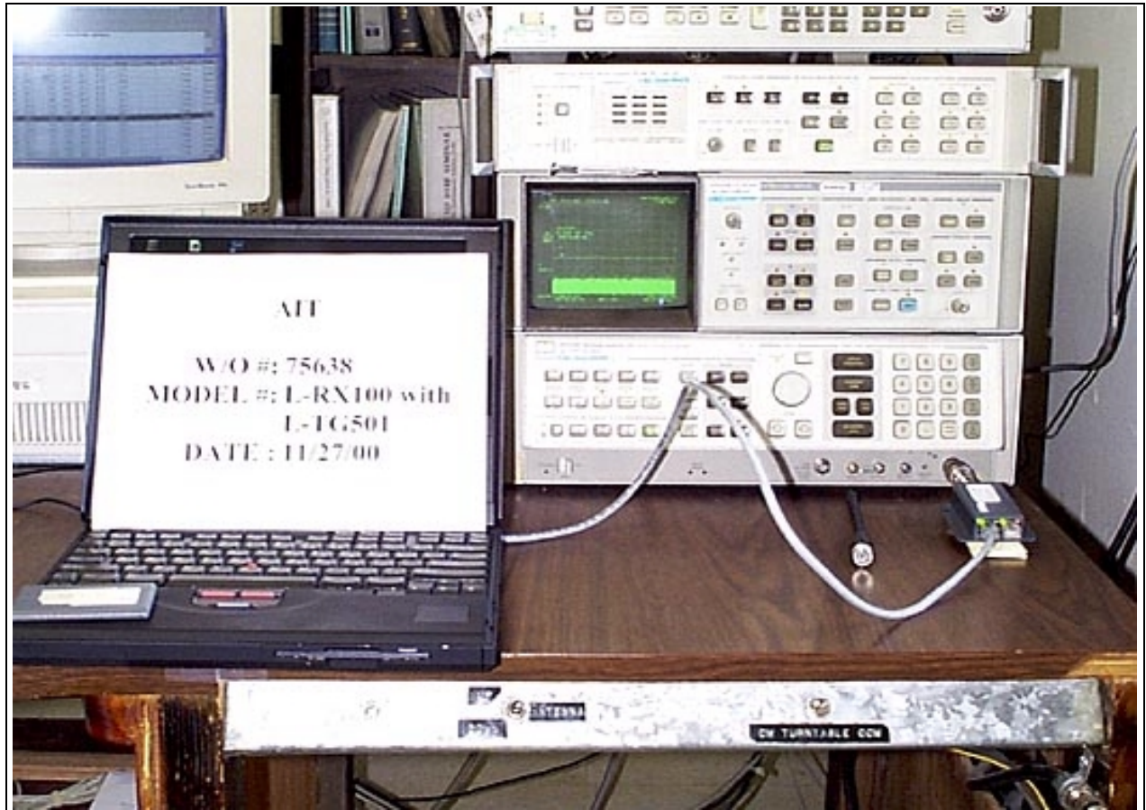
Antenna Conducted Emissions - Front View of Receiver
