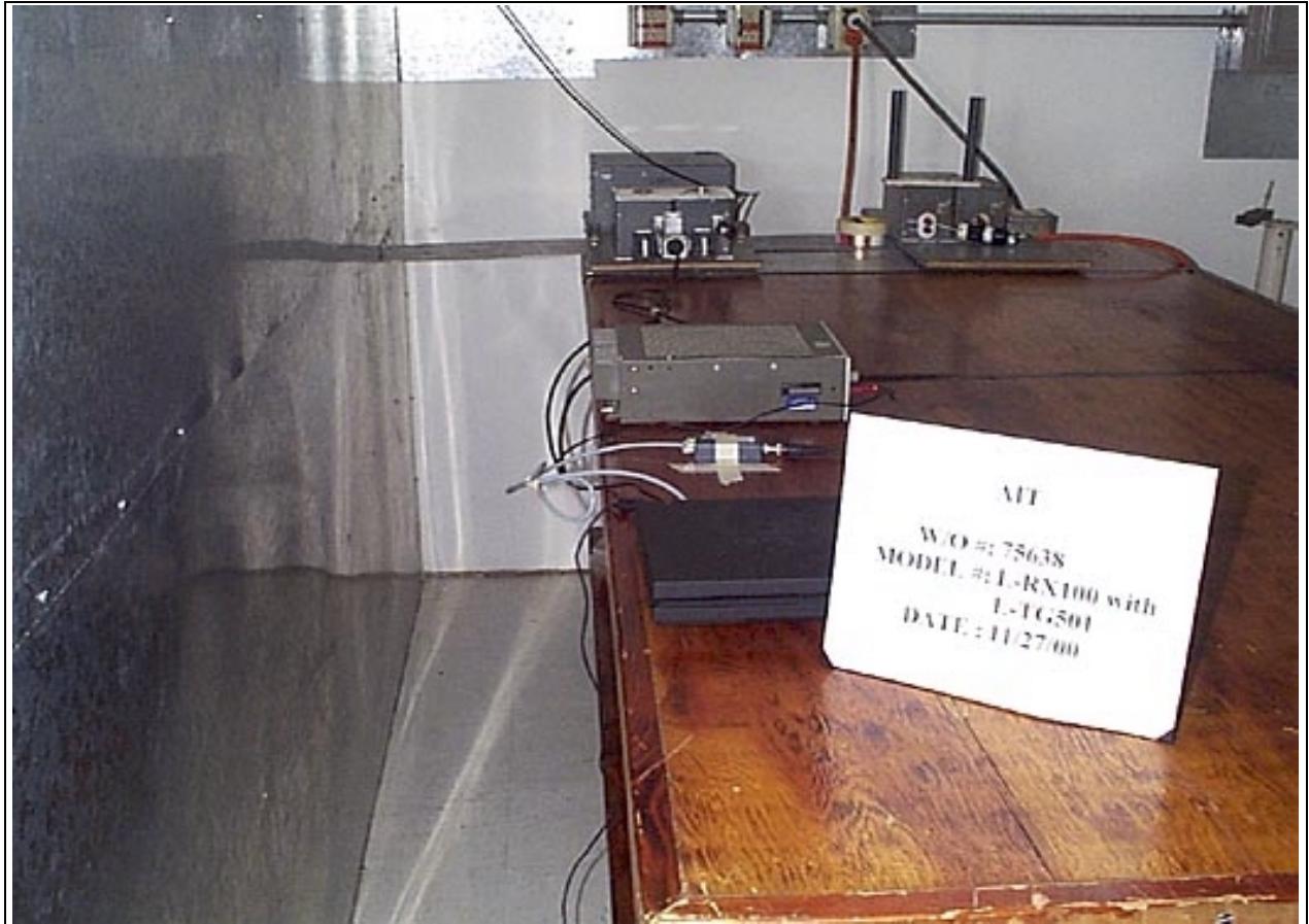
Conducted Emissions - Side View of Receiver
