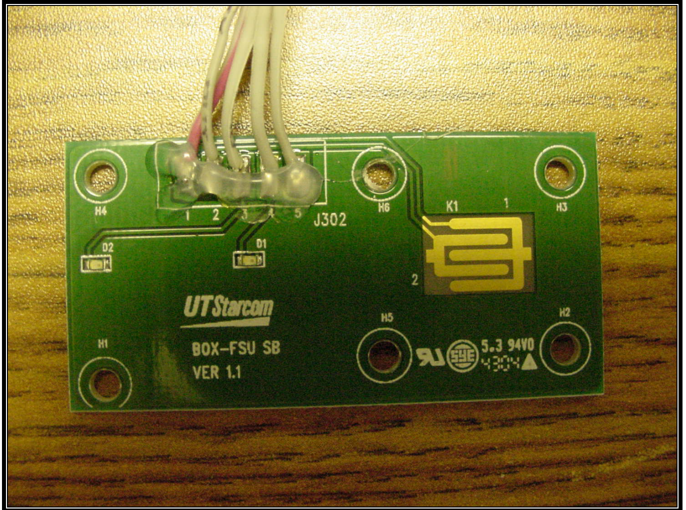
PHOTOGRAPH 16: TOP OF POWER SWITCH/LED PCB
