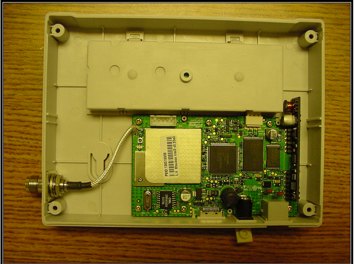
PHOTOGRAPH 18: TOP OF PCB IN BASE
