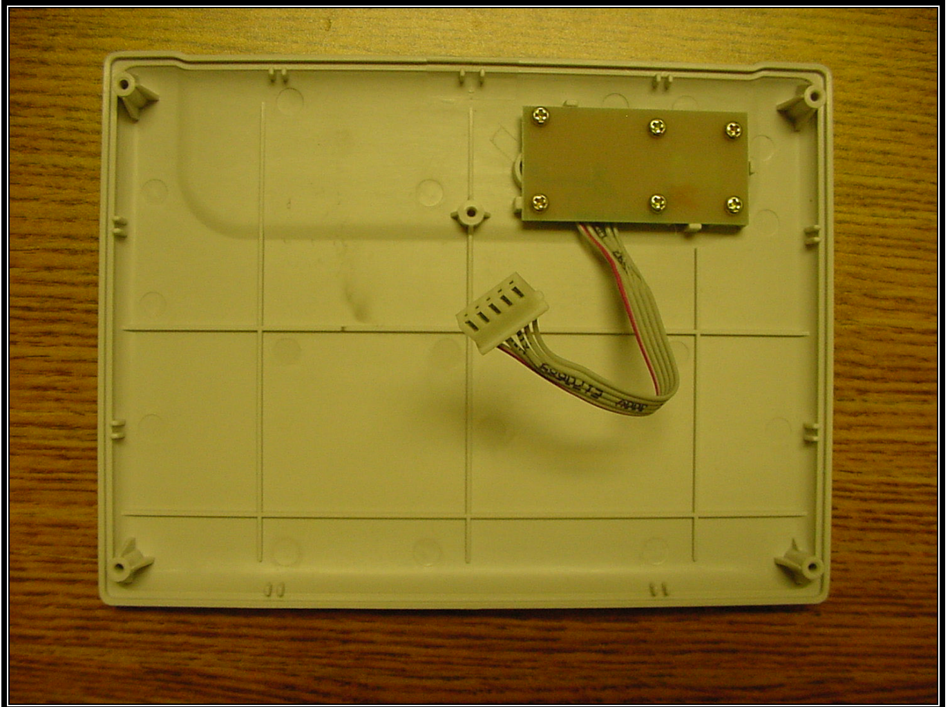
PHOTOGRAPH 17: INSIDE TOP COVER SHOWING BACK SIDE OF POWER SWITCH/LED PCB
