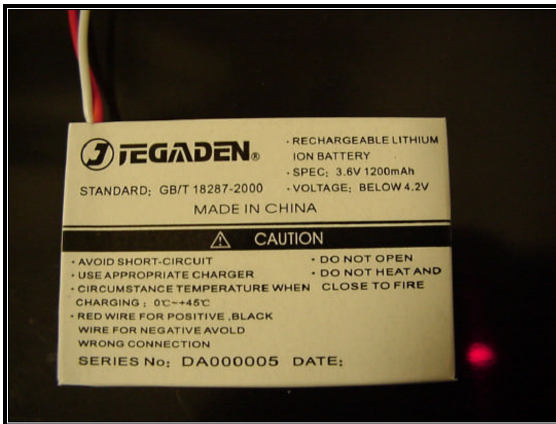
PHOTOGRAPH 10: BATTERY
