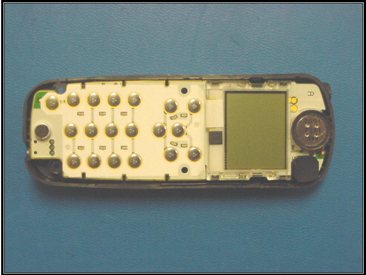
PHOTOGRAPH 19: PCB FRONT
