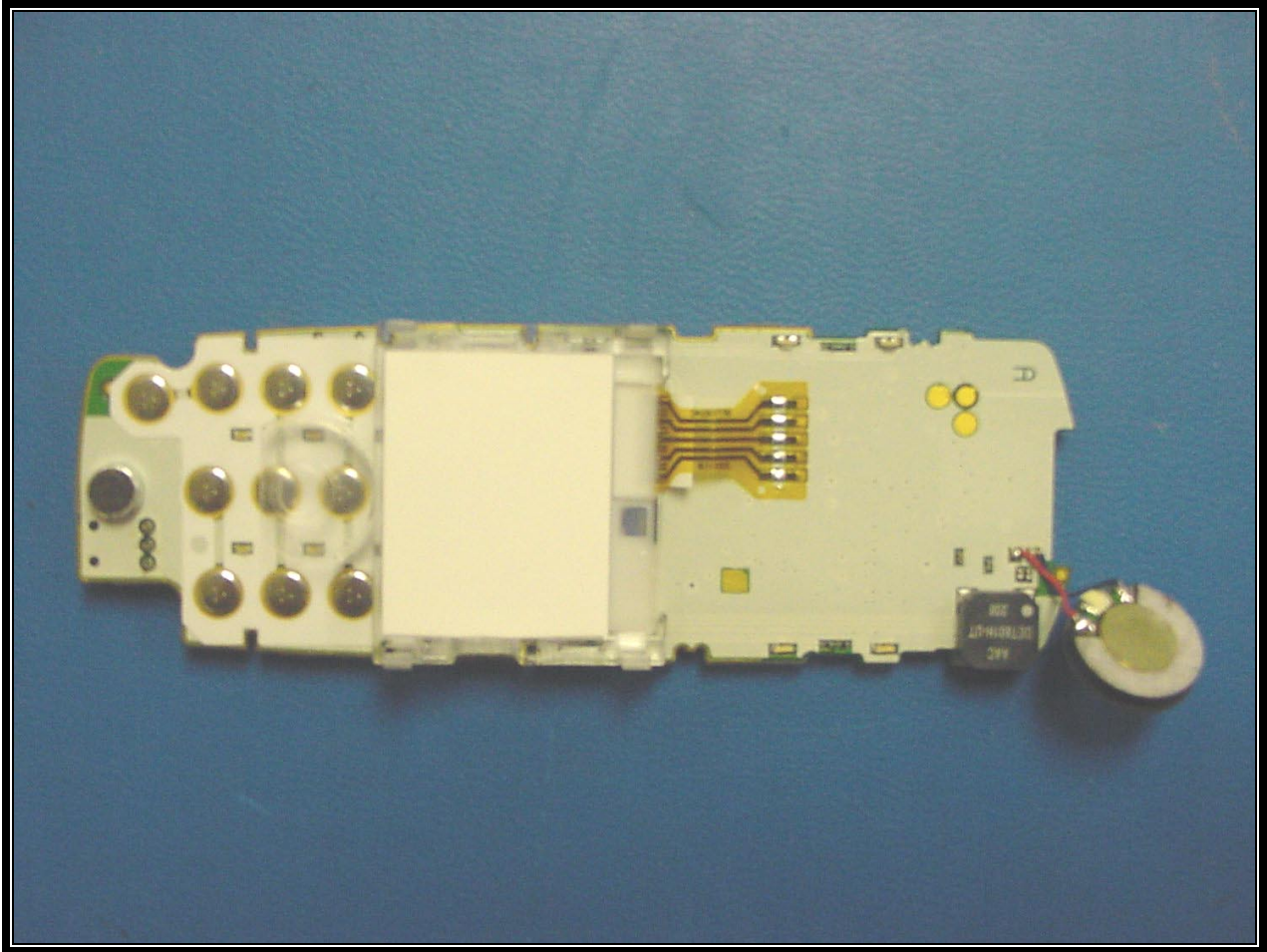
PHOTOGRAPH 22: LCD BACK
