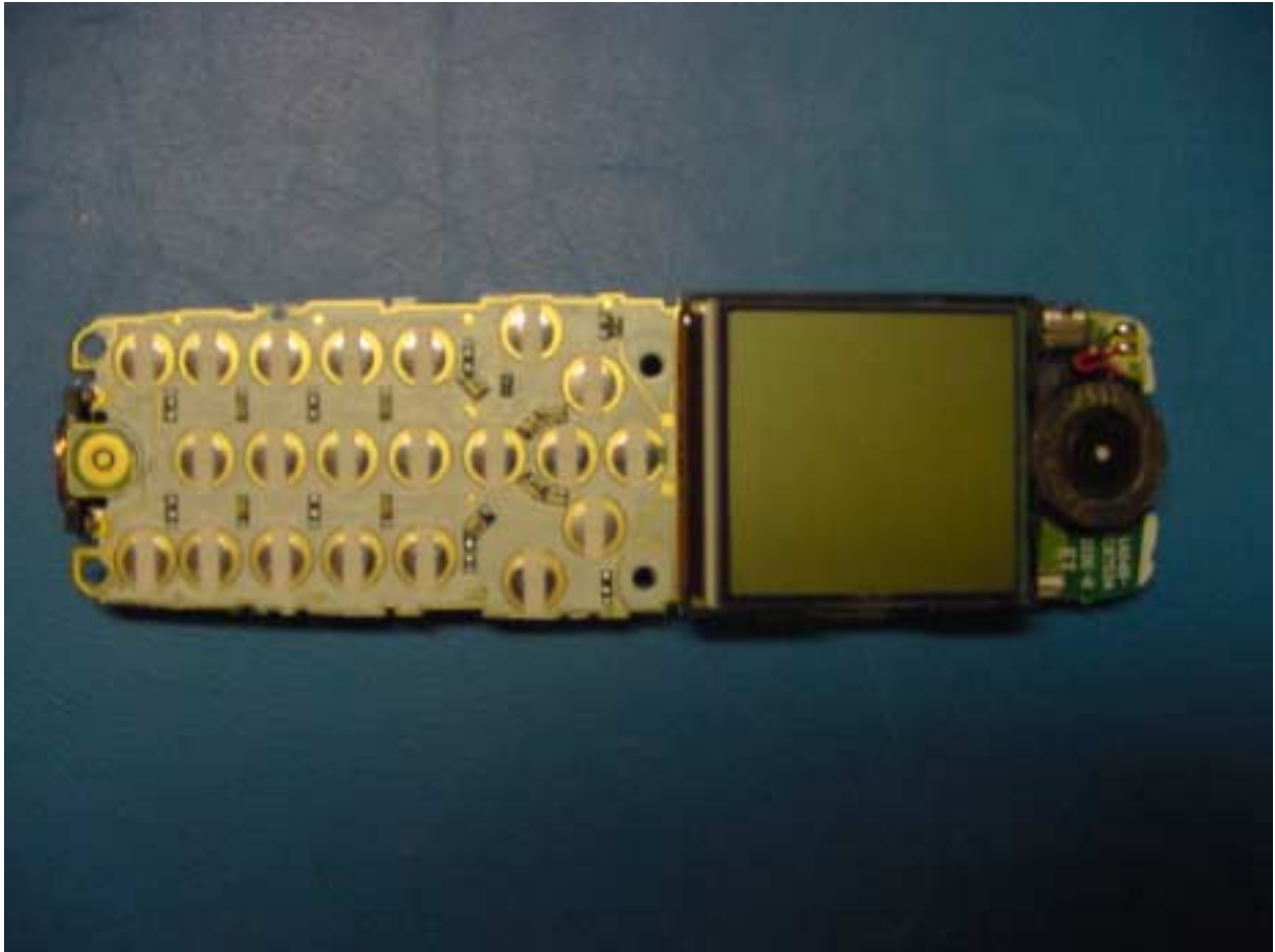
PHOTOGRAPH 9: MAIN BOARD FRONT LCD
