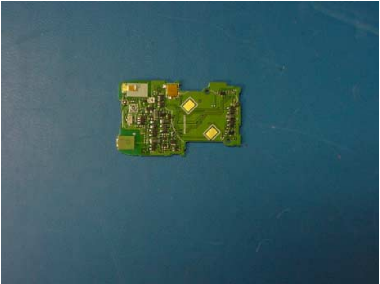
PHOTOGRAPH 13: SECONDARY REAR WITH SHIELDS
