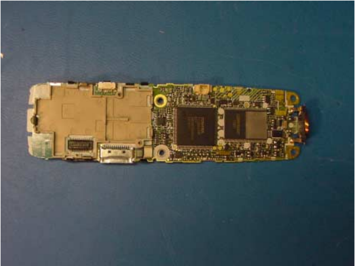
PHOTOGRAPH 10: MAIN REAR WITHOUT SECONDARY BOARD
