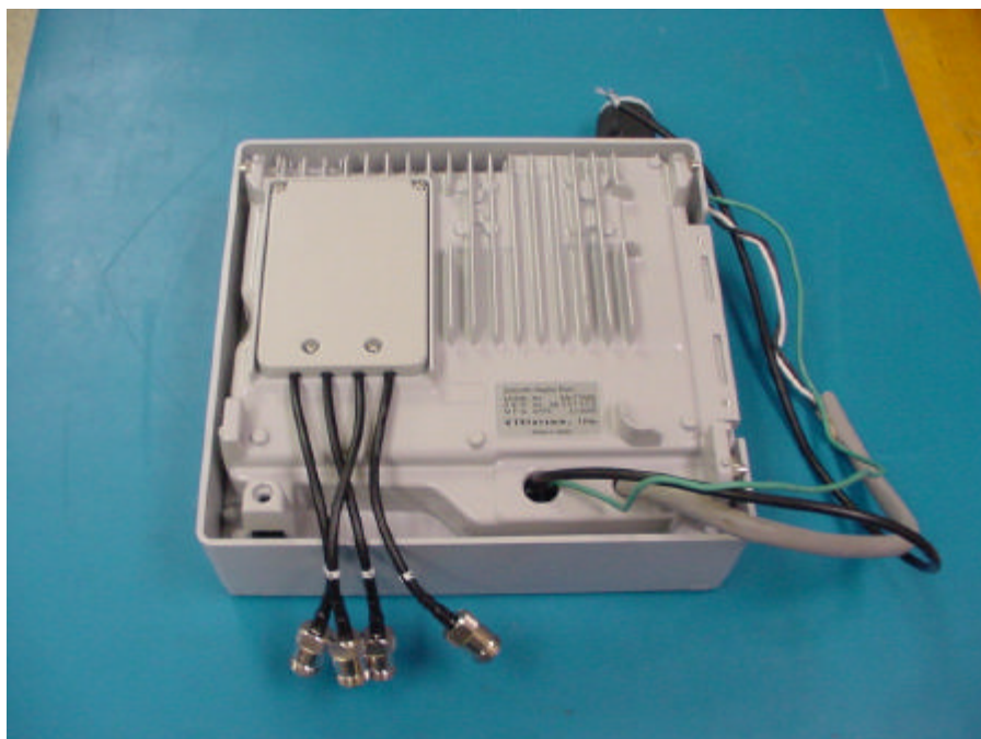
Bottom View With Cover
