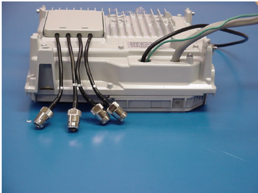
Rear View Without Cover
