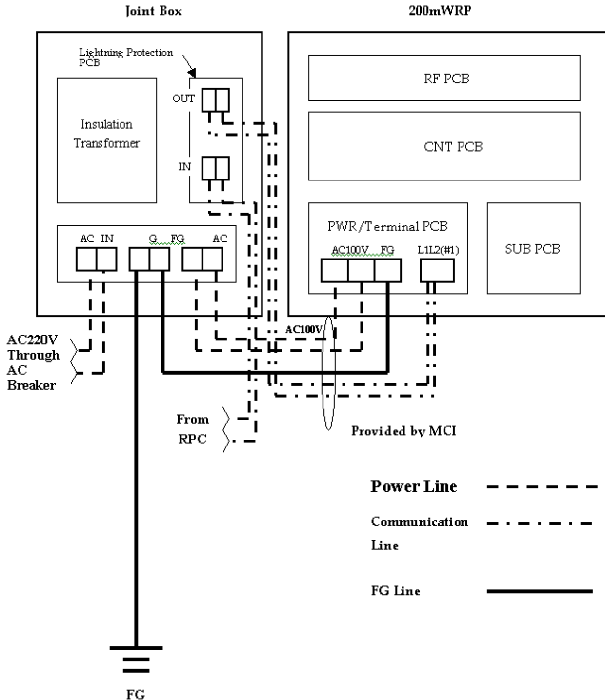
Figure 36: Electric Connection
