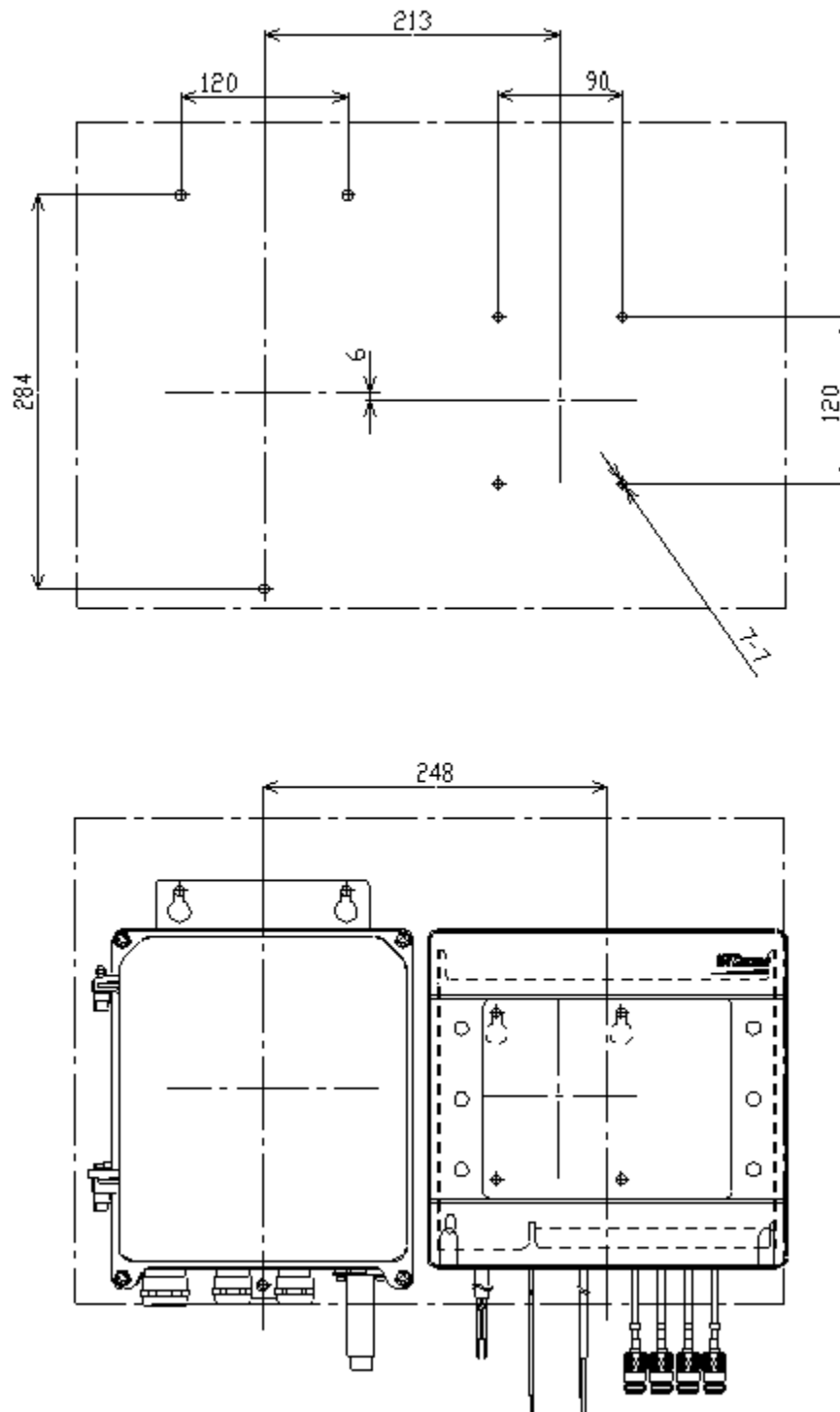
Figure 37: Layout Dimension
