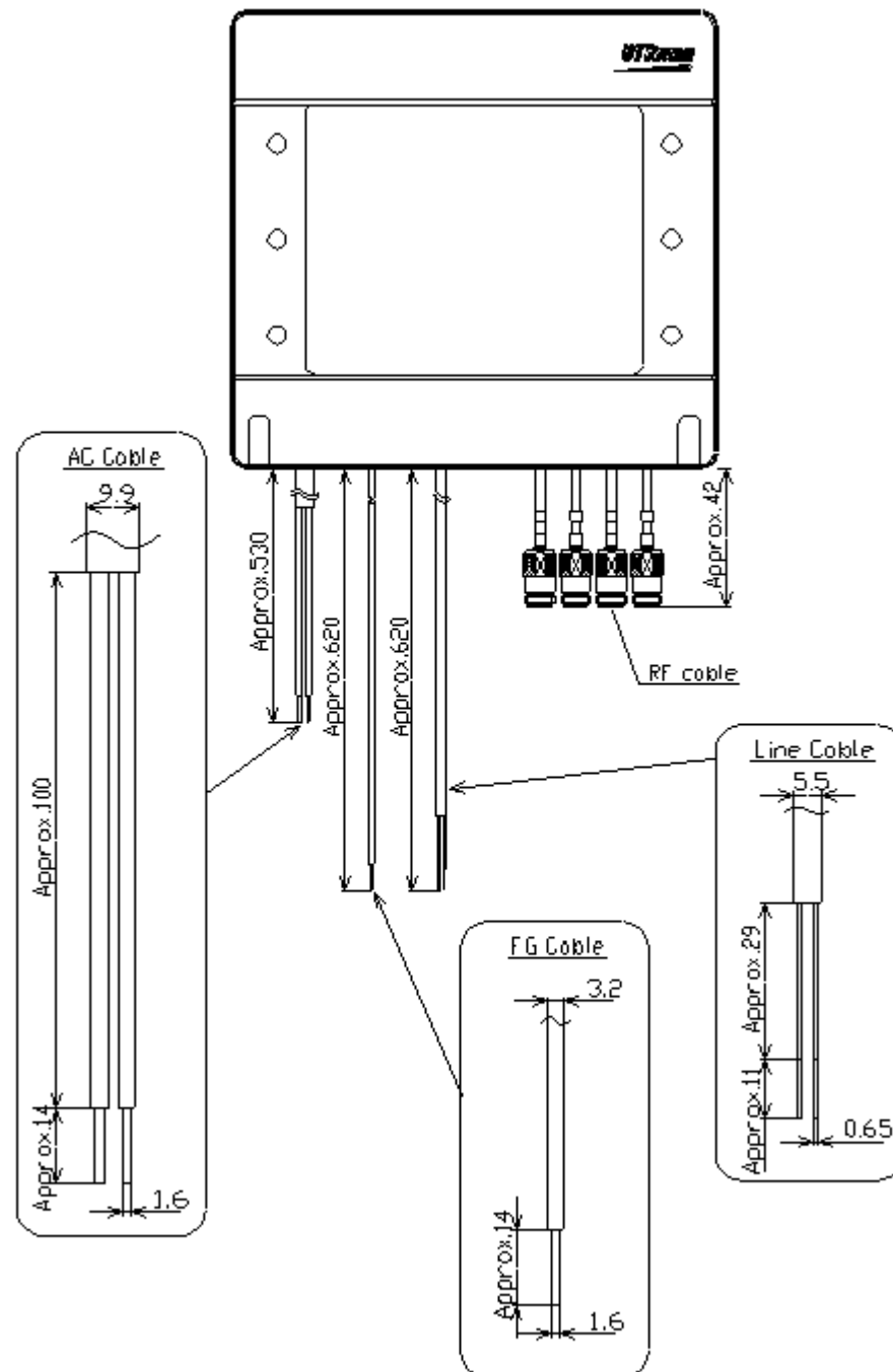
Figure 34: Cable Length
