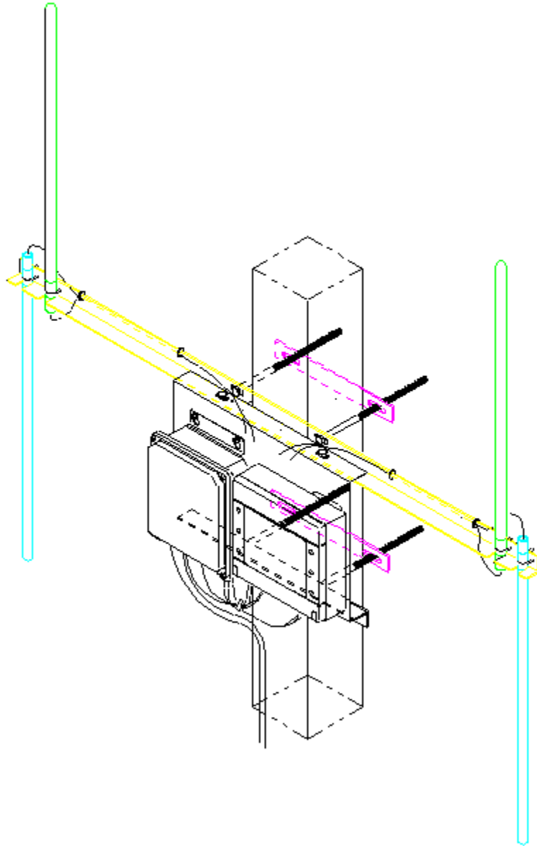
Figure 43: Pole Installation (1)
