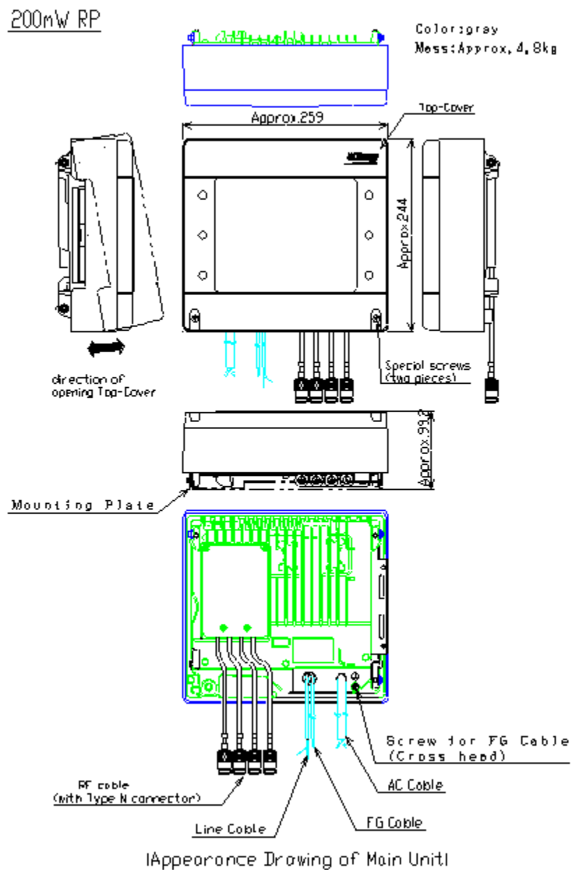
Figure 2: 200mW RP Main Unit
