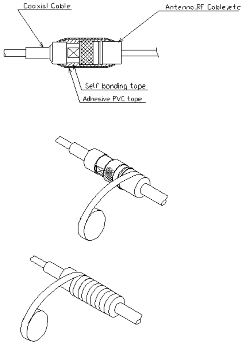
Figure 41: Water Proof of Antenna Cable (Continued)
