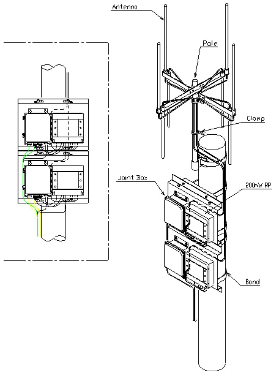
Figure 44: Pole Installation (2)
