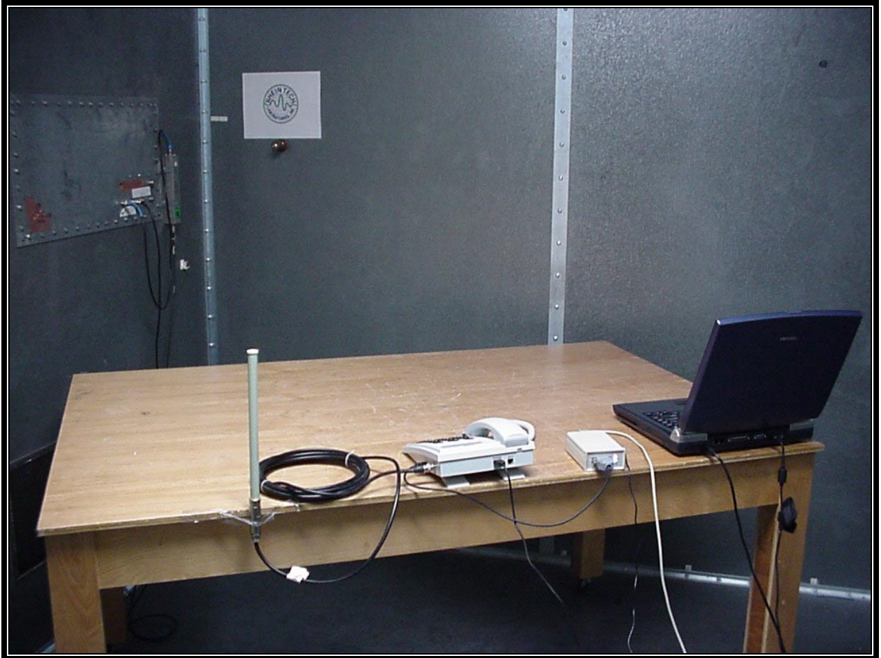
PHOTOGRAPH 13: CONDUCTED BACK VIEW WITH ROD ANTENNA
