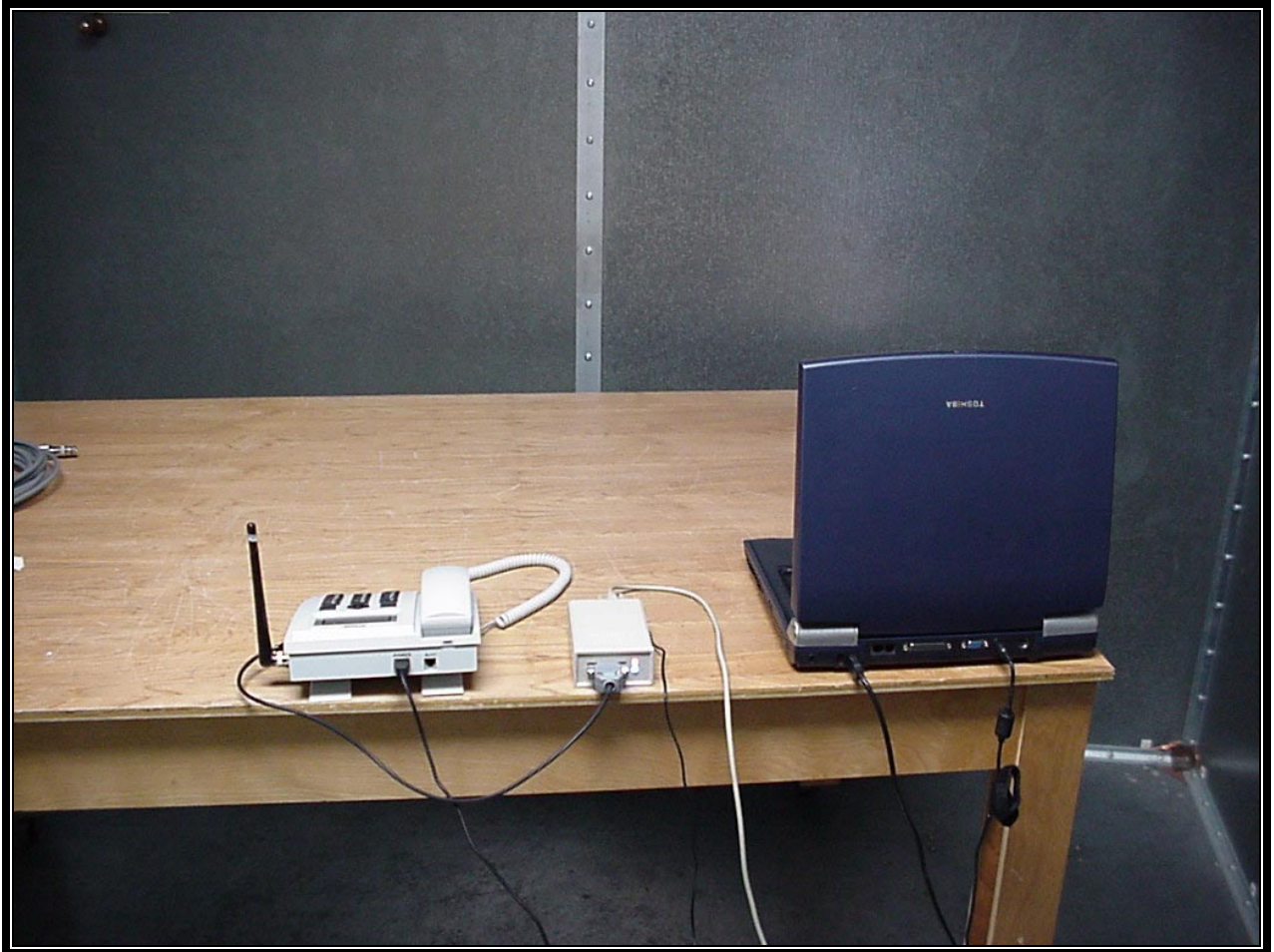
PHOTOGRAPH 9: CONDUCTED BACK VIEW WITH WHIP ANTENNA
