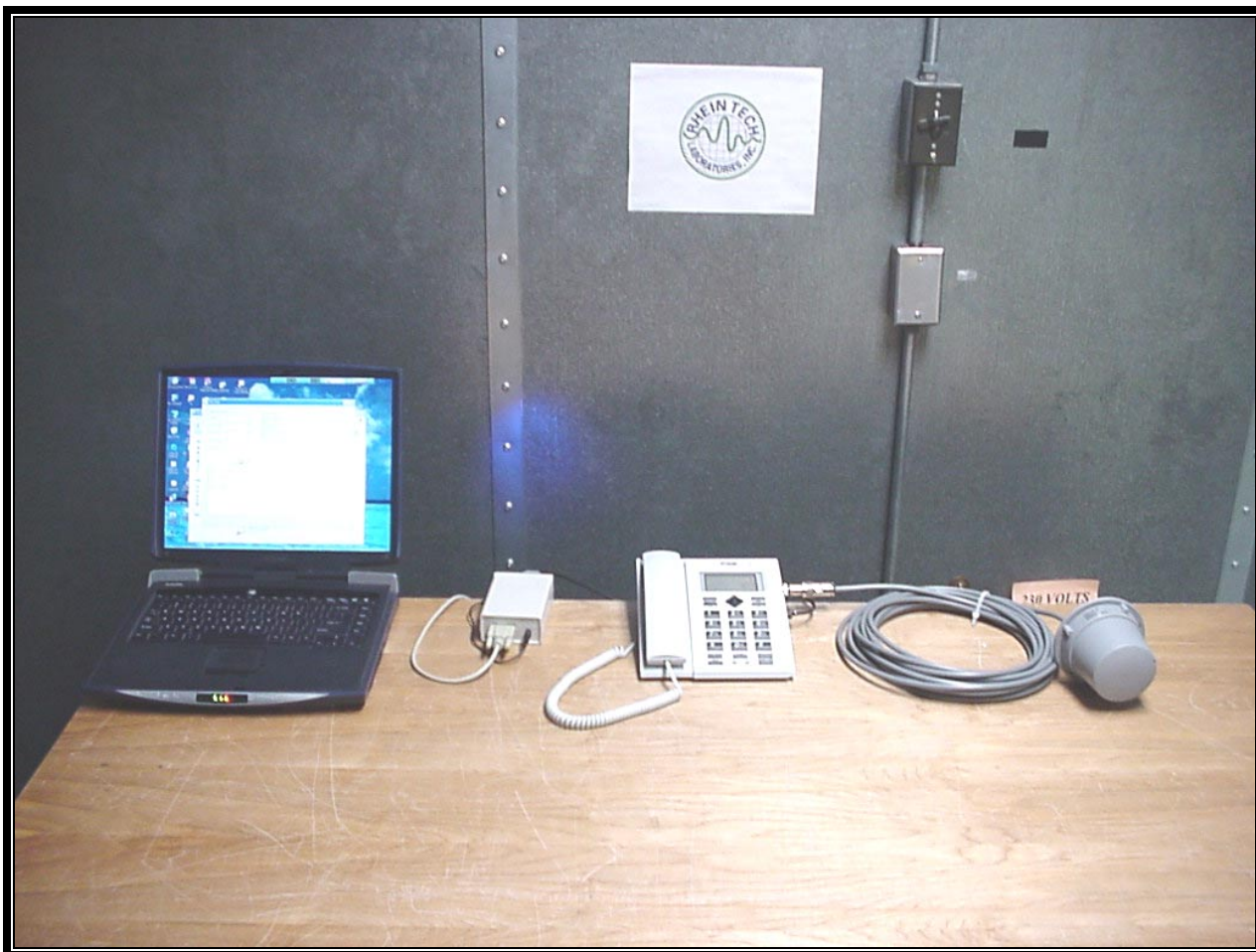
PHOTOGRAPH 10: CONDUCTED FRONT VIEW WITH PATCH ANTENNA
