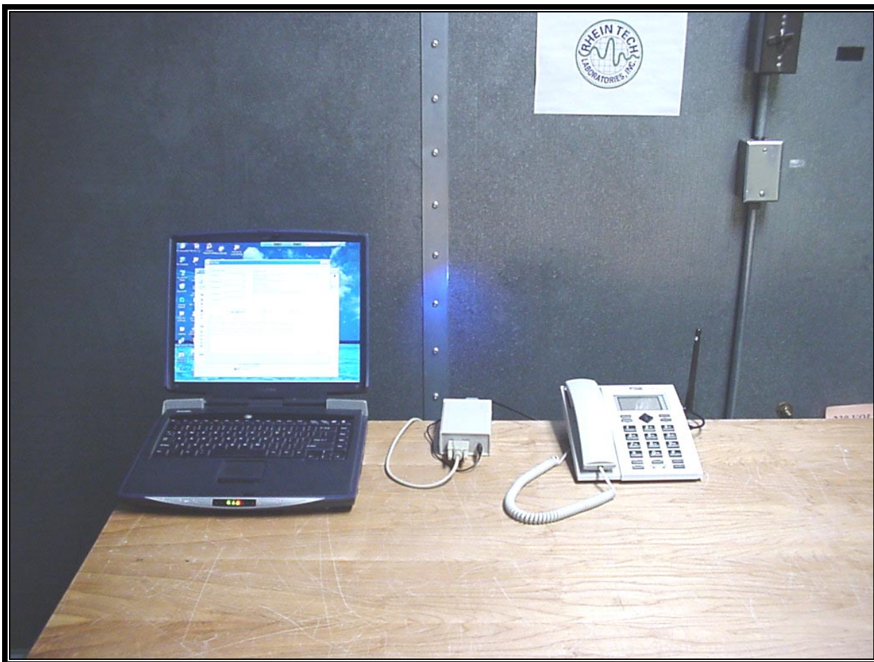
PHOTOGRAPH 8: CONDUCTED FRONT VIEW WITH WHIP ANTENNA
