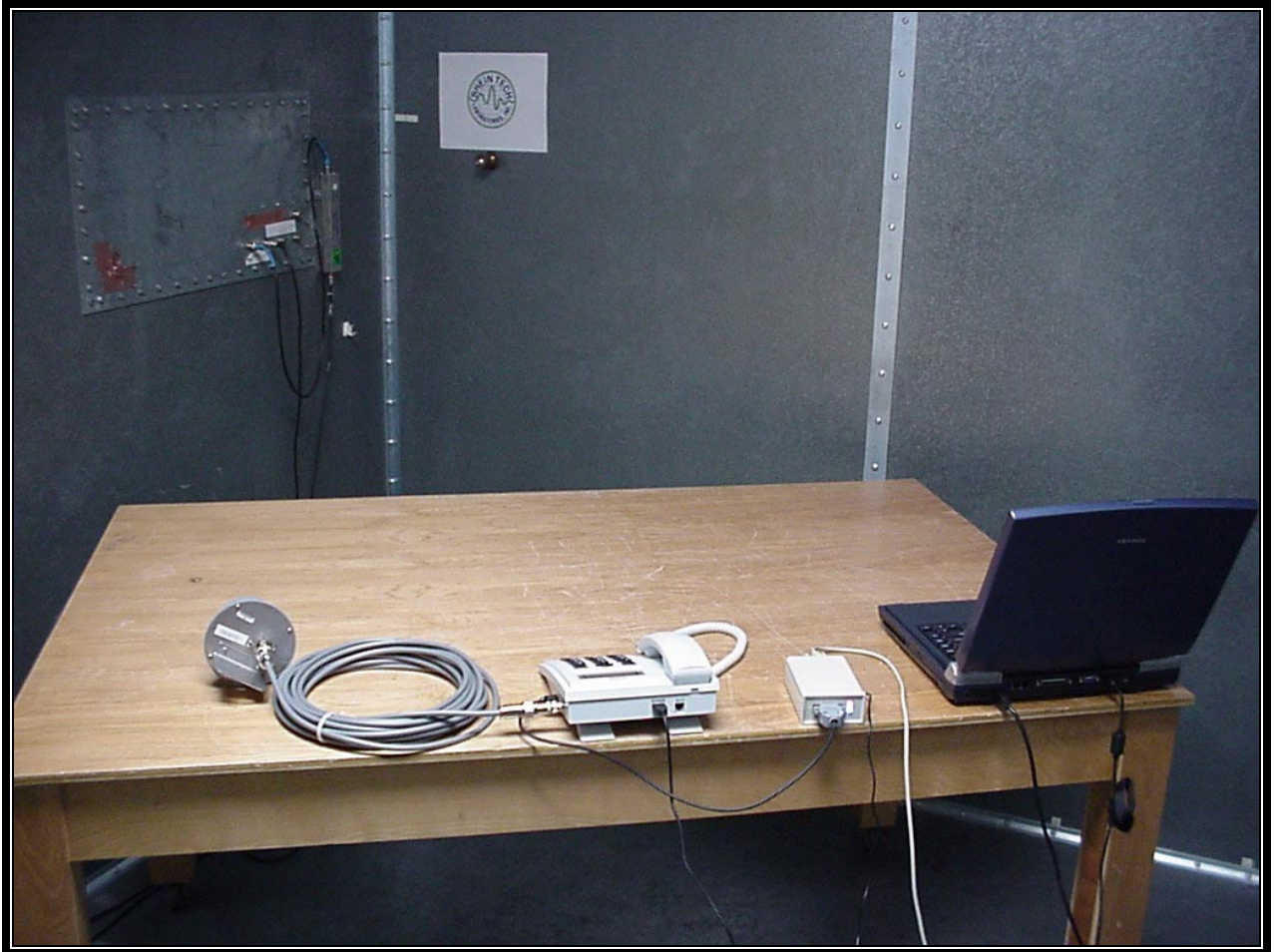
PHOTOGRAPH 11: CONDUCTED BACK VIEW WITH PATCH ANTENNA
