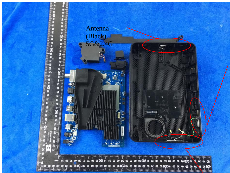
2.4G&5G Antenna View
