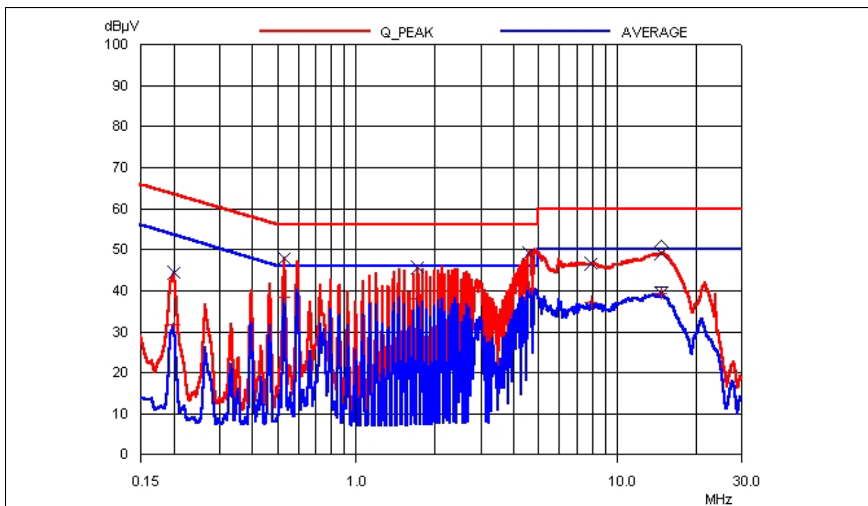
HOT LINE
