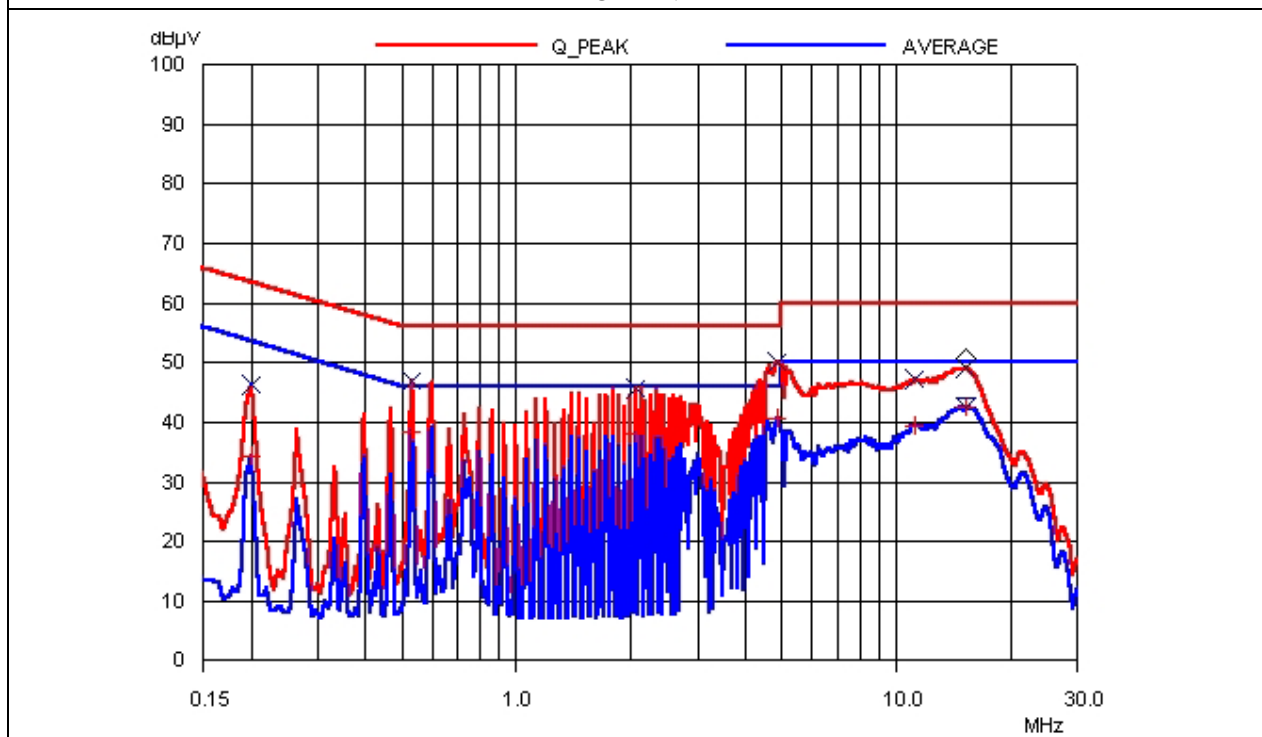
NEUTRAL LINE
