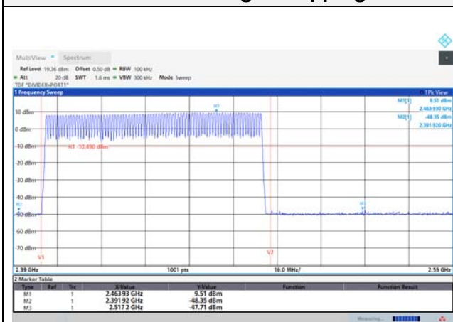
Conducted band-edge / Hopping ch.
