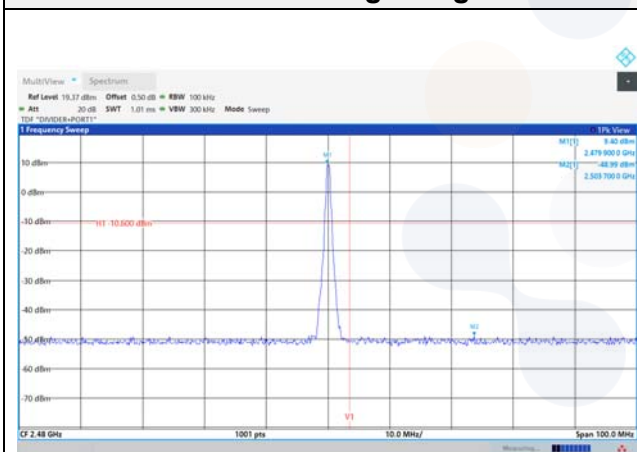
Conducted band-edge / High ch.
