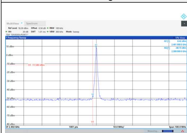
Conducted band-edge / Low ch.
