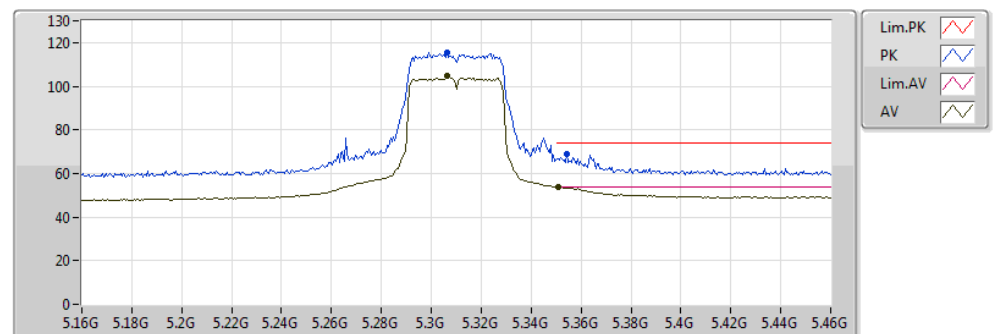
RE TX above 1GHz;Band:5.3G;VHT40,BF;BWch:40MHz;Nss:2,(M0);Nant:4;Ch:5310MHz;TX
