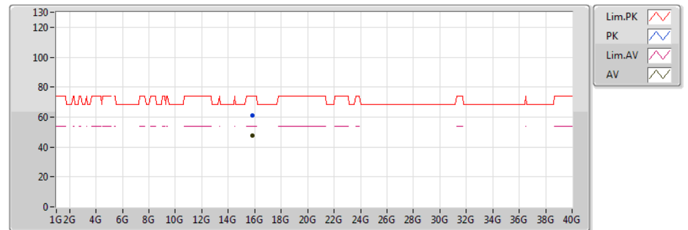
RE TX above 1GHz;Band:5.3G;VHT40,BF;BWch:40MHz;Nss:2,(M0);Nant:4;Ch:5270MHz;TX
