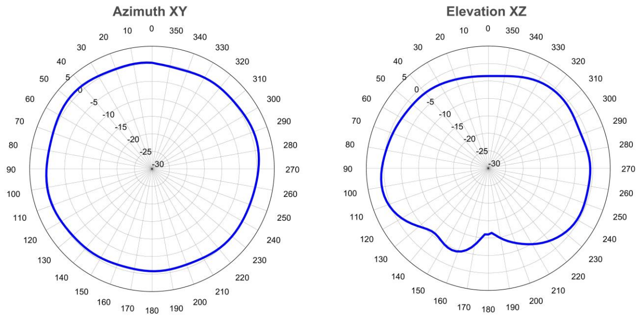
Figure 3: Model N24X2H2YW Measured Radiation Patterns at 2.44 GHz
