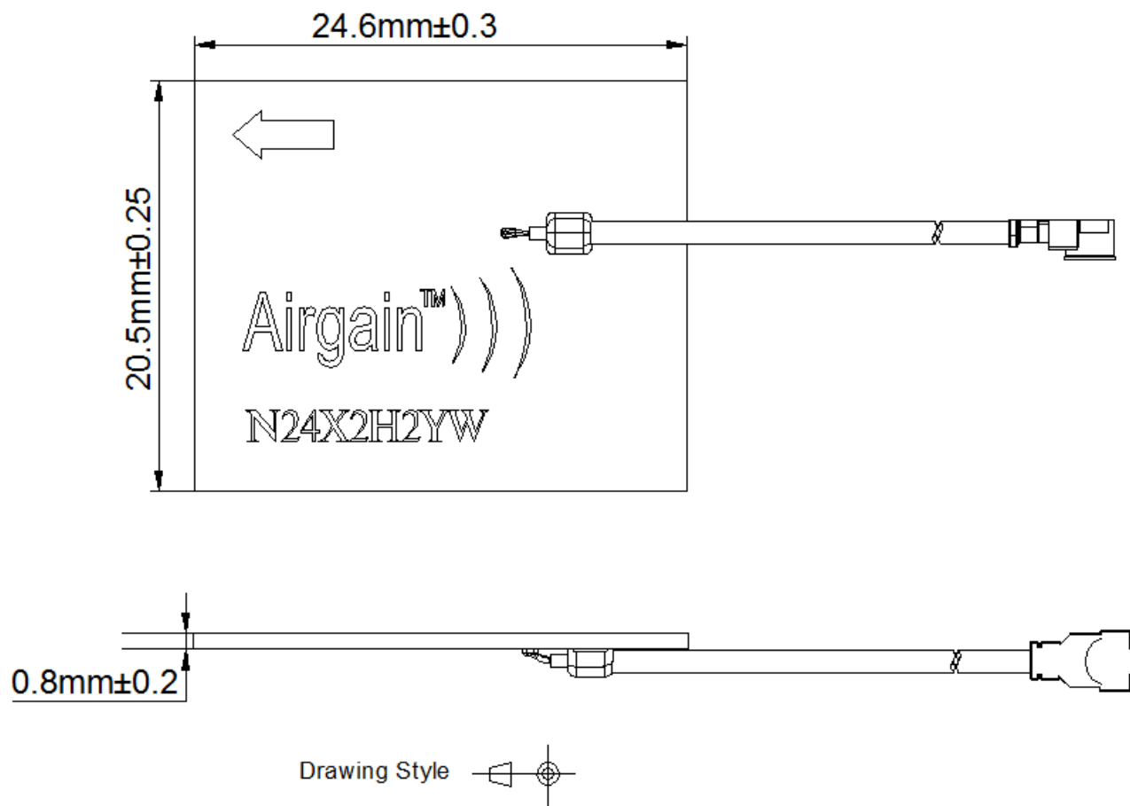
Figure 6: Model N24X2H2YW Embedded Antenna Dimensions
