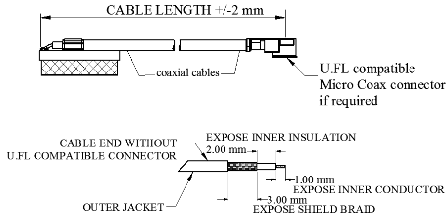
Figure 7: N24X2H2YW with connector or stripped cable
