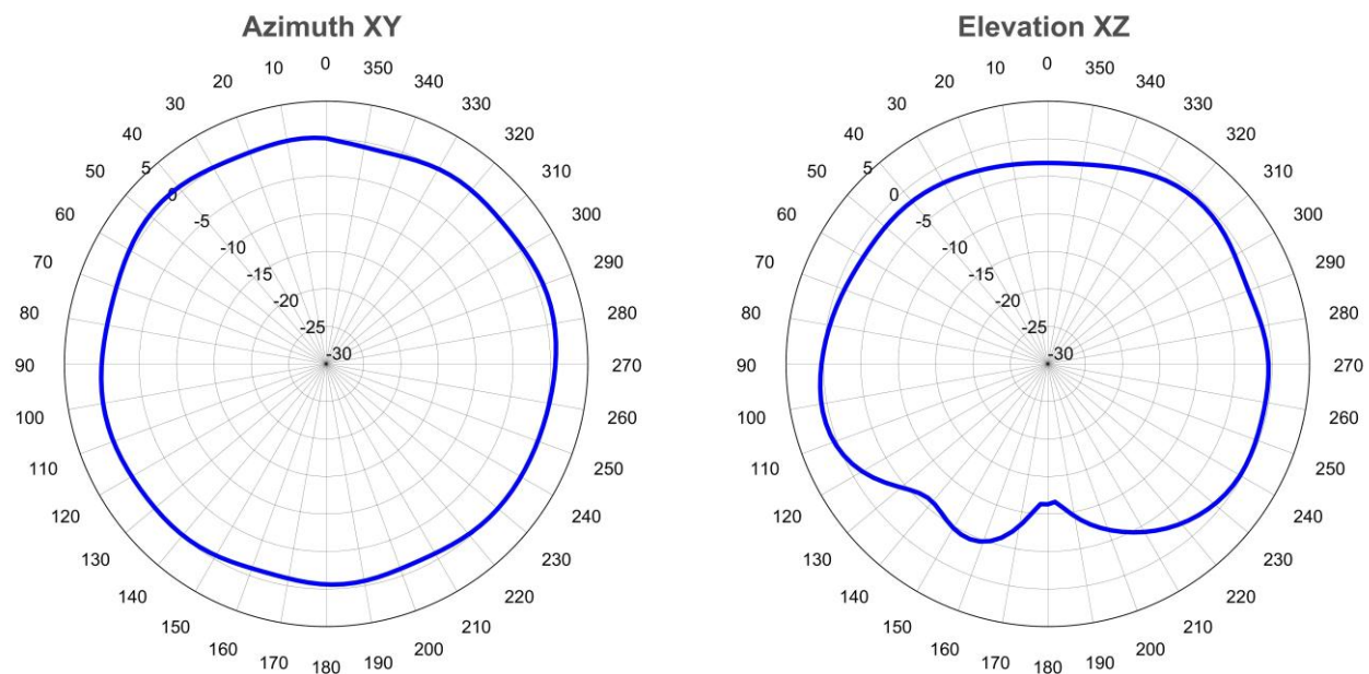
Figure 5: Model N24X2H2YW Measured Radiation Patterns at 2.44 GHz
