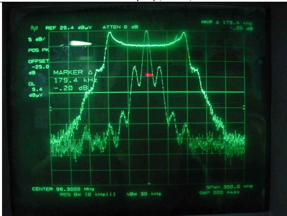
Middle Frequency (98.3MHz)
