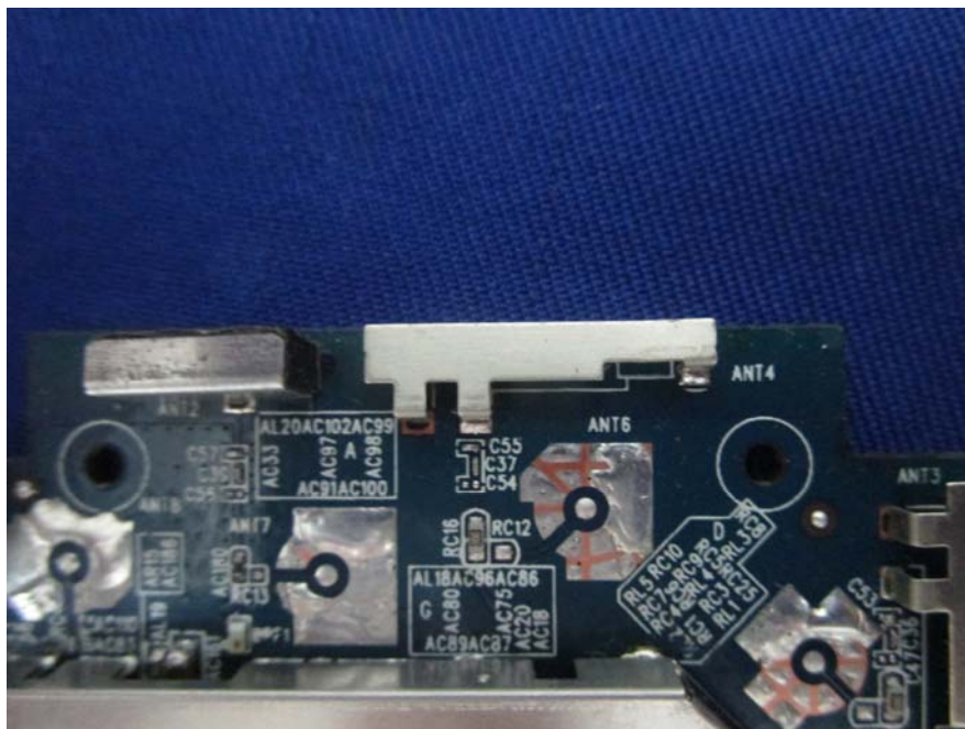
EUT – 2.4G ANT3 View
