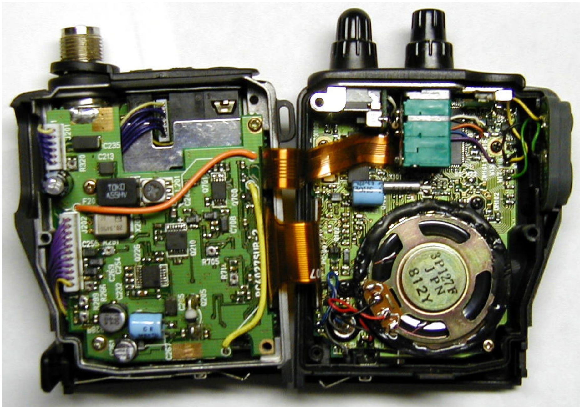
Sub-Board Top Side
