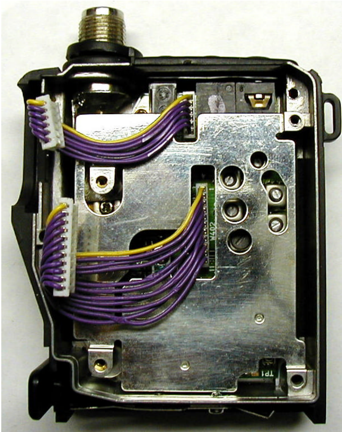
RF Board with Shield in Place
