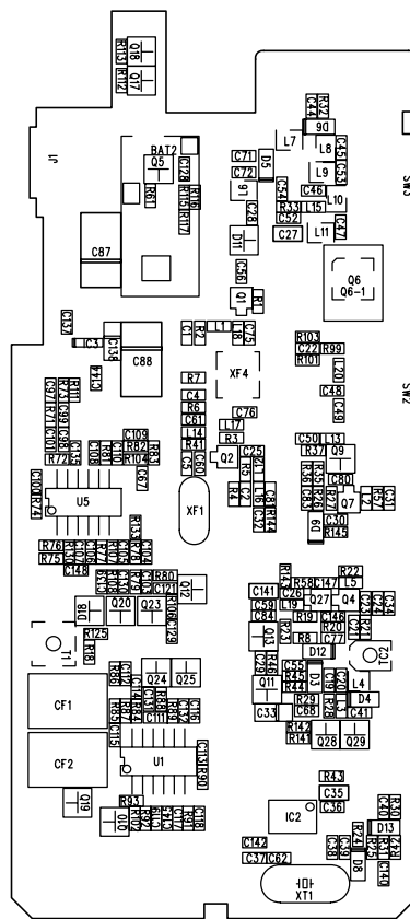
BOTTOM SILKSCREEN
