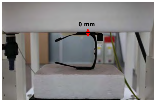
Fig.3 Position the outside of the arm against the phantom(Plot 1)
