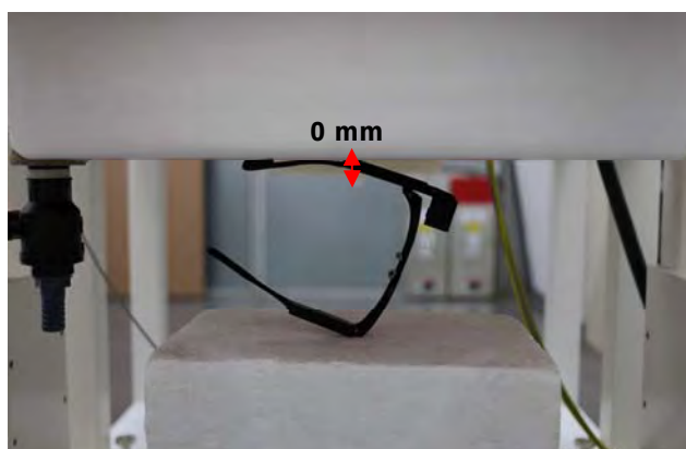
Fig.4 Position the outside of the arm against the phantom(Plot 2)
