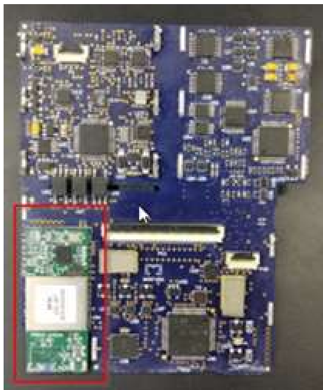
Top of Host Device PCB, with Module Board Outlined (*note: there are no components beneath module board)
