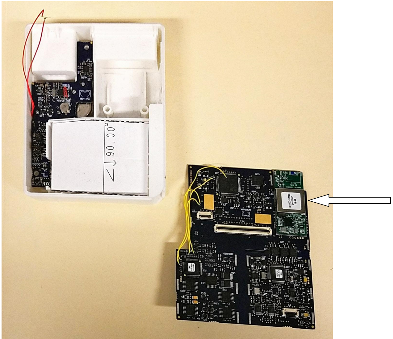
Internal Photos of Host Device (arrow points to module board)
