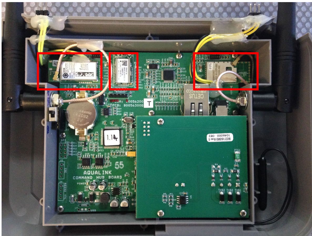
Figure 2. Modules on Evaluation Board
