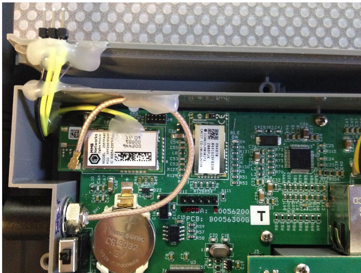
Figure 4. Co-Located Radio Modules on Evaluation Board
