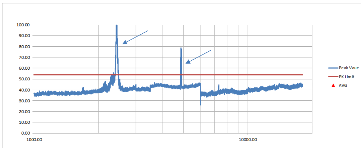
Figure 6. Vertical Radiated Emissions above 1 GHz
